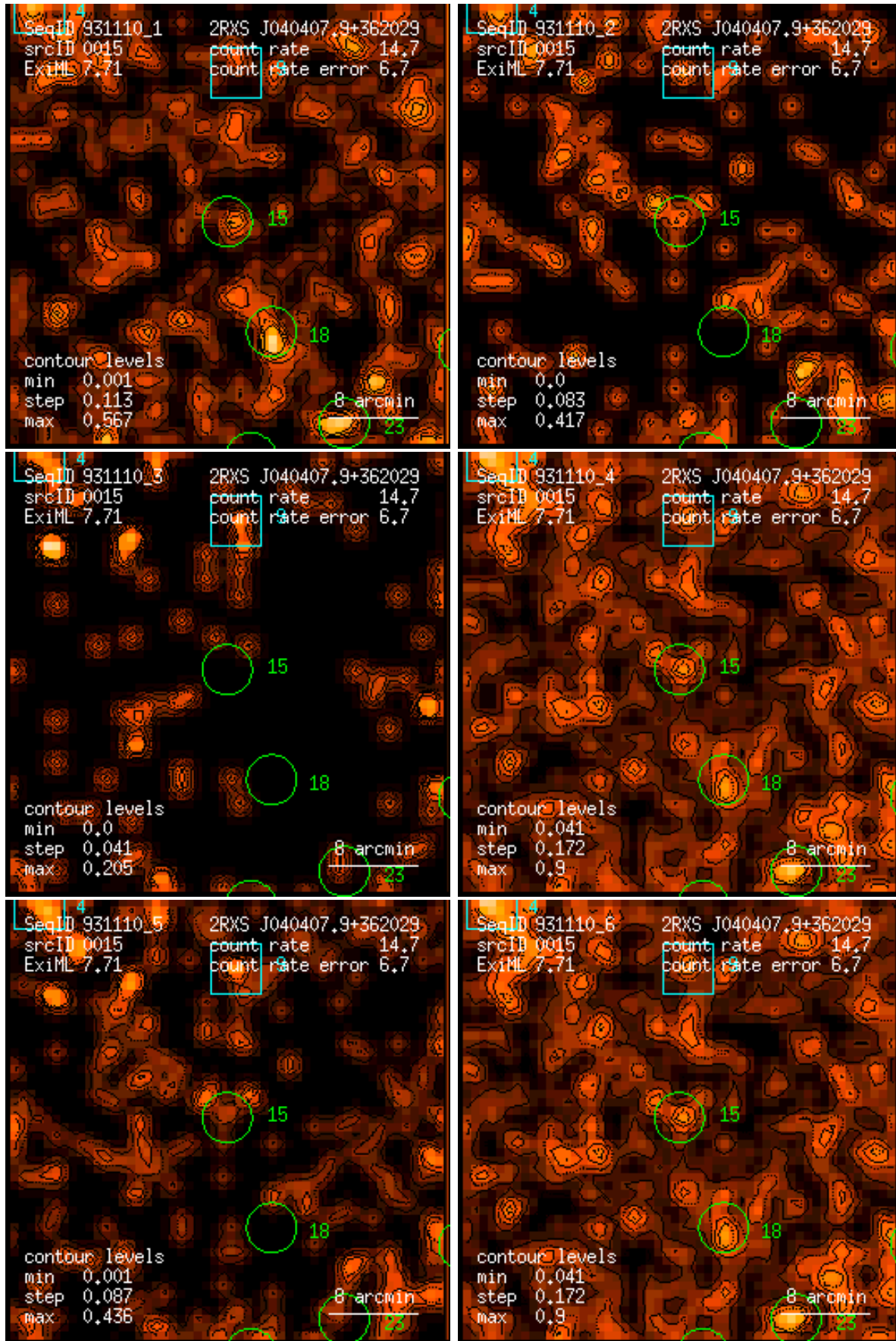
Figure 15: RASS 931110: detection 0015: band rate images, Gaussian filter: (1) PSPC channels 11 – 41, (2) 52 – 90, (3) 91 – 201, (4) 11 – 235, (5) 52 – 201, (6) 11 – 201. Broad band rates in counts/ks. Band rate contour levels in counts/ks/arcmin 2 .
