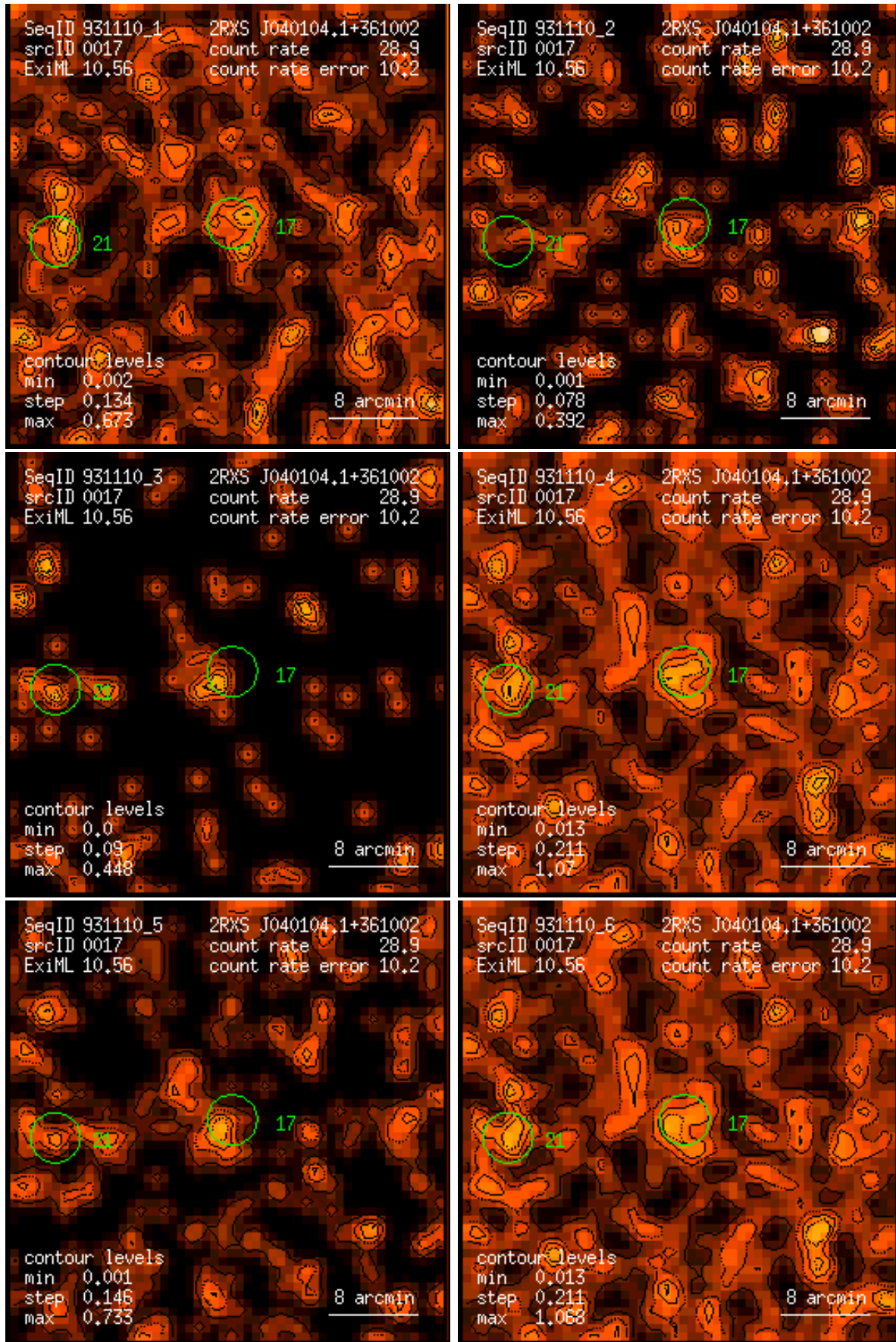
Figure 17: RASS 931110: detection 0017: band rate images, Gaussian filter: (1) PSPC channels 11 – 41, (2) 52 – 90, (3) 91 – 201, (4) 11 – 235, (5) 52 – 201, (6) 11 – 201. Broad band rates in counts/ks. Band rate contour levels in counts/ks/arcmin 2 .
