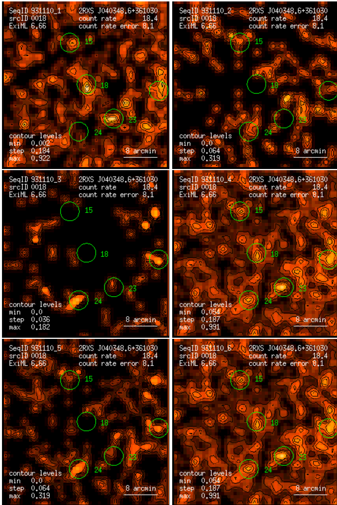
Figure 18: RASS 931110: detection 0018: band rate images, Gaussian filter: (1) PSPC channels 11 – 41, (2) 52 – 90, (3) 91 – 201, (4) 11 – 235, (5) 52 – 201, (6) 11 – 201. Broad band rates in counts/ks. Band rate contour levels in counts/ks/arcmin 2 .
