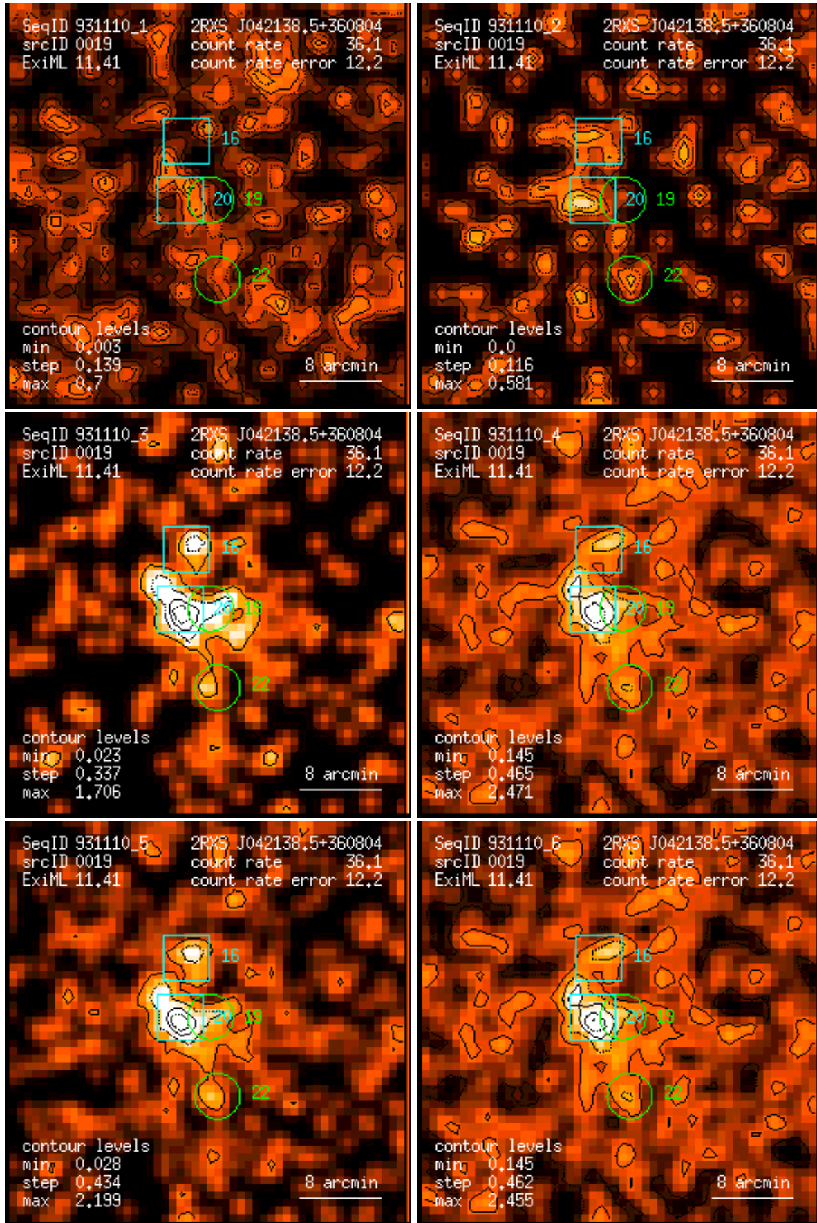
Figure 19: RASS 931110: detection 0019: band rate images, Gaussian filter: (1) PSPC channels 11 – 41, (2) 52 – 90, (3) 91 – 201, (4) 11 – 235, (5) 52 – 201, (6) 11 – 201. Broad band rates in counts/ks. Band rate contour levels in counts/ks/arcmin 2 .
