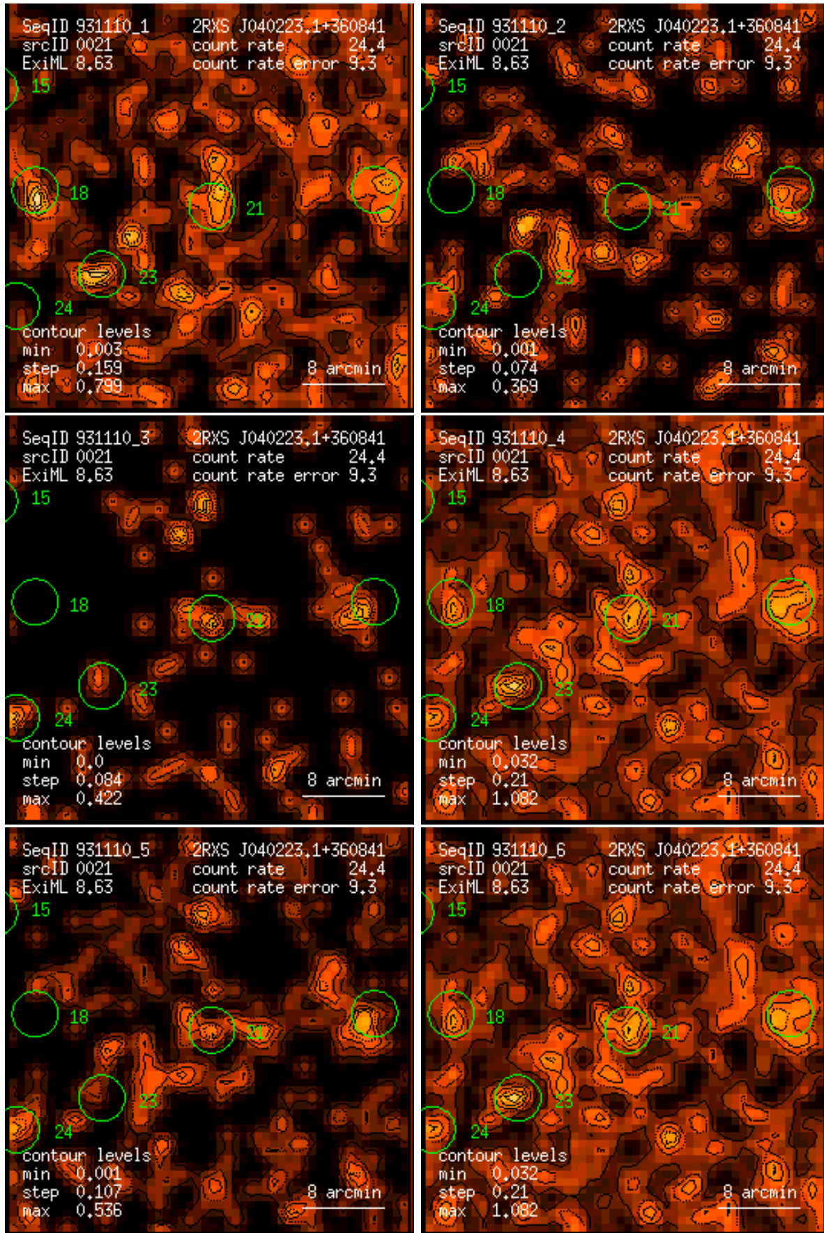
Figure 21: RASS 931110: detection 0021: band rate images, Gaussian filter: (1) PSPC channels 11 – 41, (2) 52 – 90, (3) 91 – 201, (4) 11 – 235, (5) 52 – 201, (6) 11 – 201. Broad band rates in counts/ks. Band rate contour levels in counts/ks/arcmin 2 .
