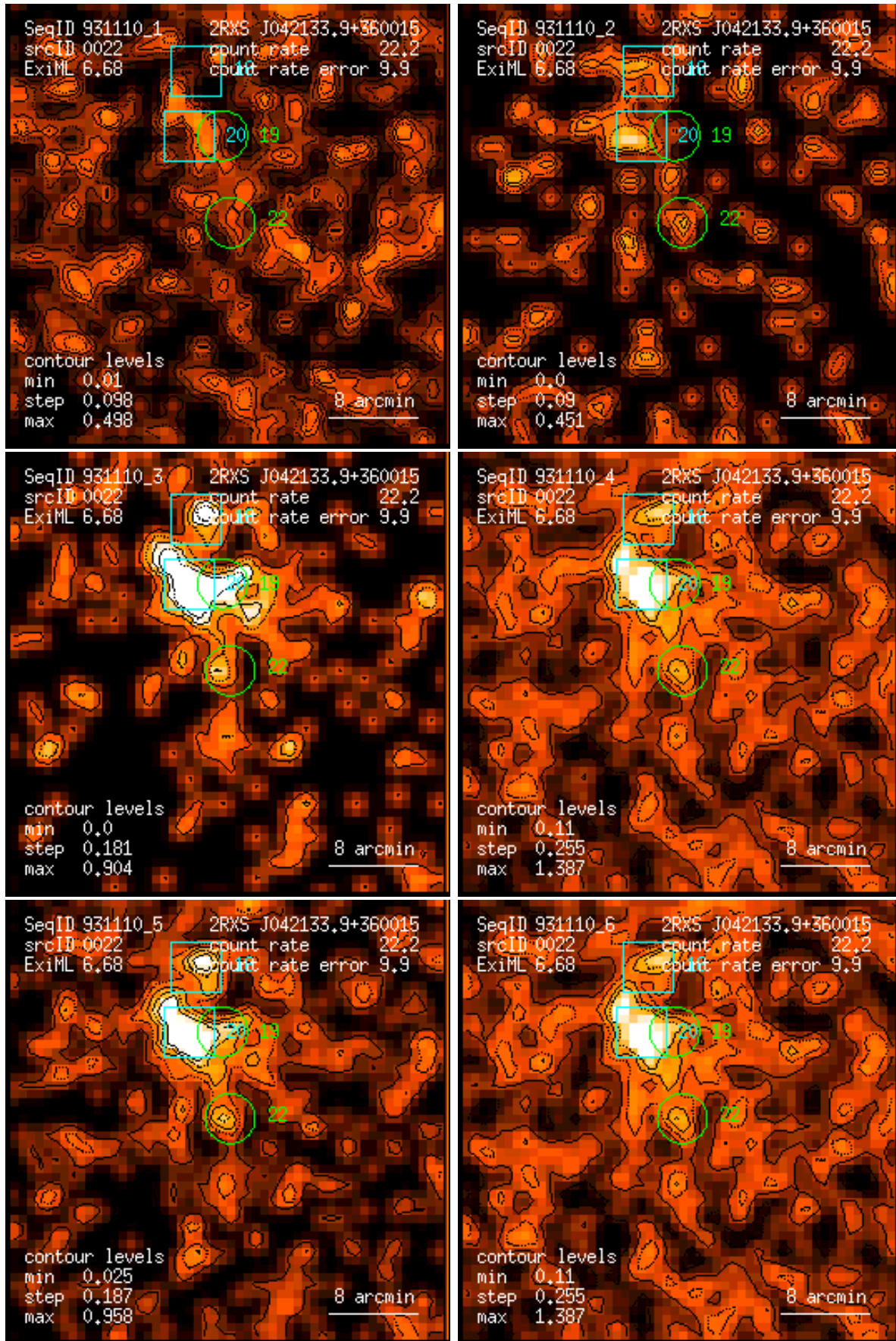
Figure 22: RASS 931110: detection 0022: band rate images, Gaussian filter: (1) PSPC channels 11 – 41, (2) 52 – 90, (3) 91 – 201, (4) 11 – 235, (5) 52 – 201, (6) 11 – 201. Broad band rates in counts/ks. Band rate contour levels in counts/ks/arcmin 2 .
