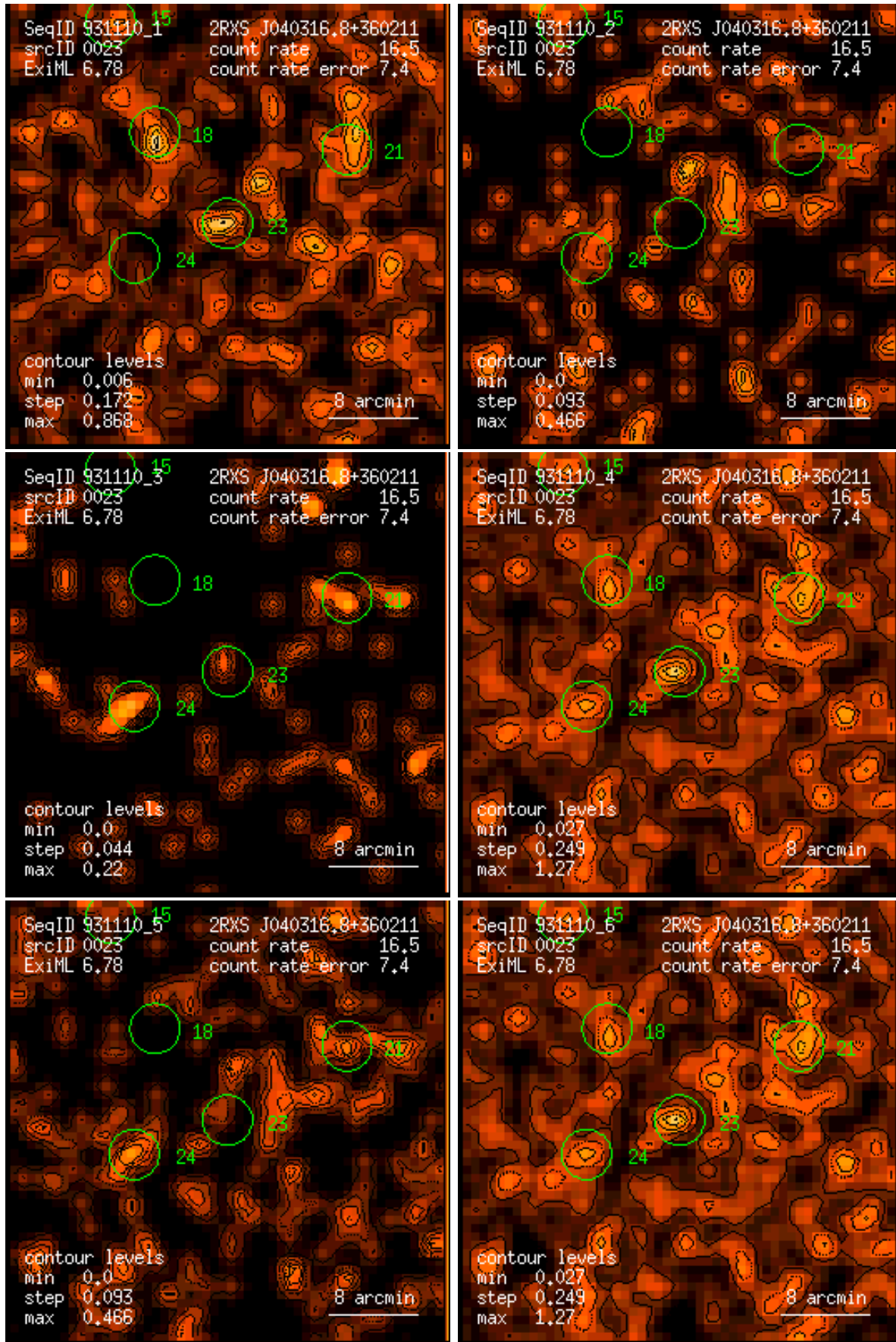
Figure 23: RASS 931110: detection 0023: band rate images, Gaussian filter: (1) PSPC channels 11 – 41, (2) 52 – 90, (3) 91 – 201, (4) 11 – 235, (5) 52 – 201, (6) 11 – 201. Broad band rates in counts/ks. Band rate contour levels in counts/ks/arcmin 2 .
