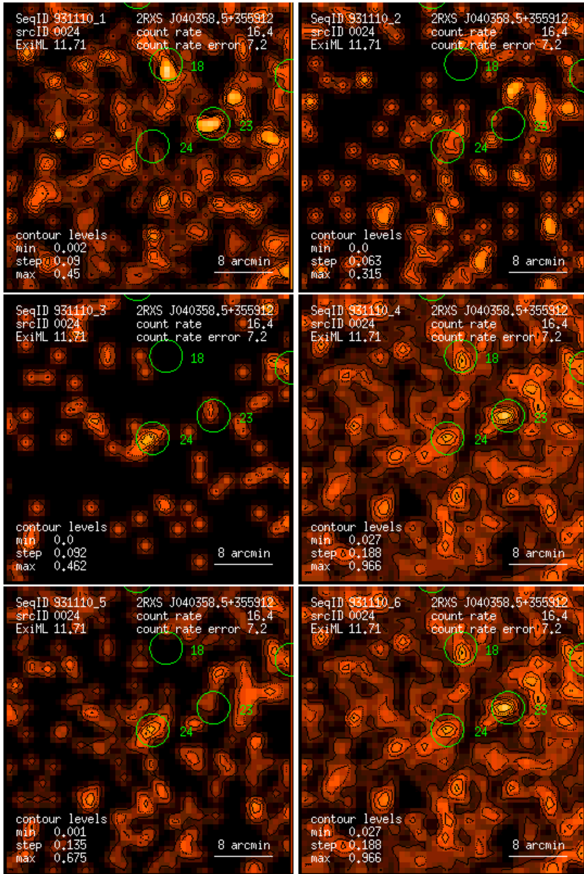
Figure 24: RASS 931110: detection 0024: band rate images, Gaussian filter: (1) PSPC channels 11 – 41, (2) 52 – 90, (3) 91 – 201, (4) 11 – 235, (5) 52 – 201, (6) 11 – 201. Broad band rates in counts/ks. Band rate contour levels in counts/ks/arcmin 2 .
