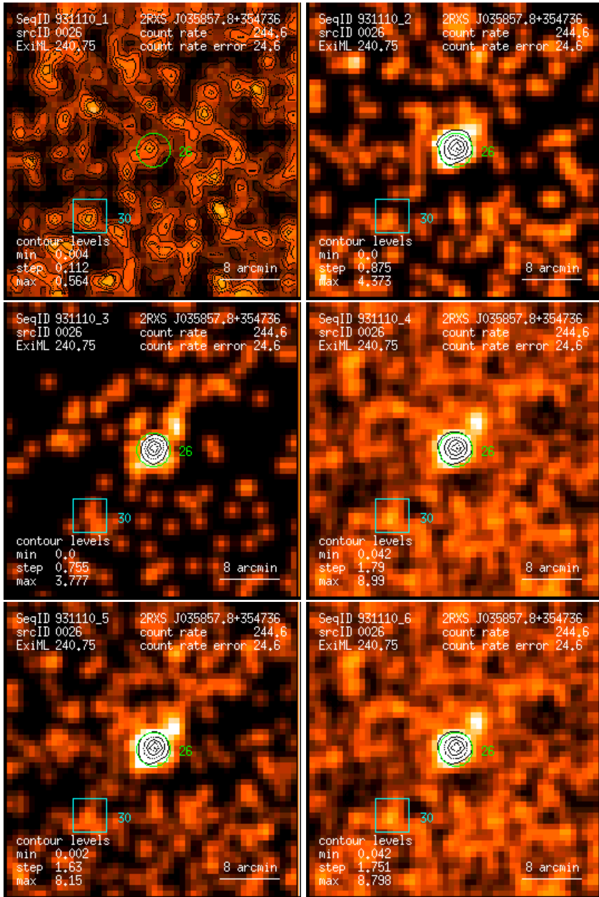
Figure 26: RASS 931110: detection 0026: band rate images, Gaussian filter: (1) PSPC channels 11 – 41, (2) 52 – 90, (3) 91 – 201, (4) 11 – 235, (5) 52 – 201, (6) 11 – 201. Broad band rates in counts/ks. Band rate contour levels in counts/ks/arcmin 2 .
