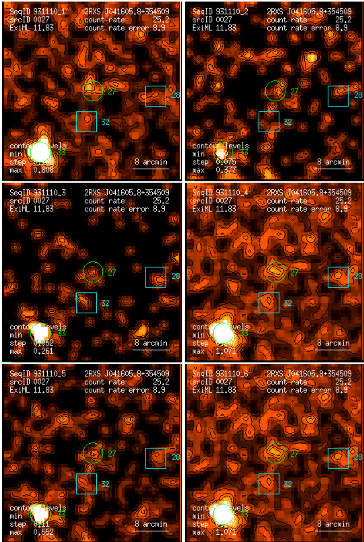
Figure 27: RASS 931110: detection 0027: band rate images, Gaussian filter: (1) PSPC channels 11 – 41, (2) 52 – 90, (3) 91 – 201, (4) 11 – 235, (5) 52 – 201, (6) 11 – 201. Broad band rates in counts/ks. Band rate contour levels in counts/ks/arcmin 2 .
