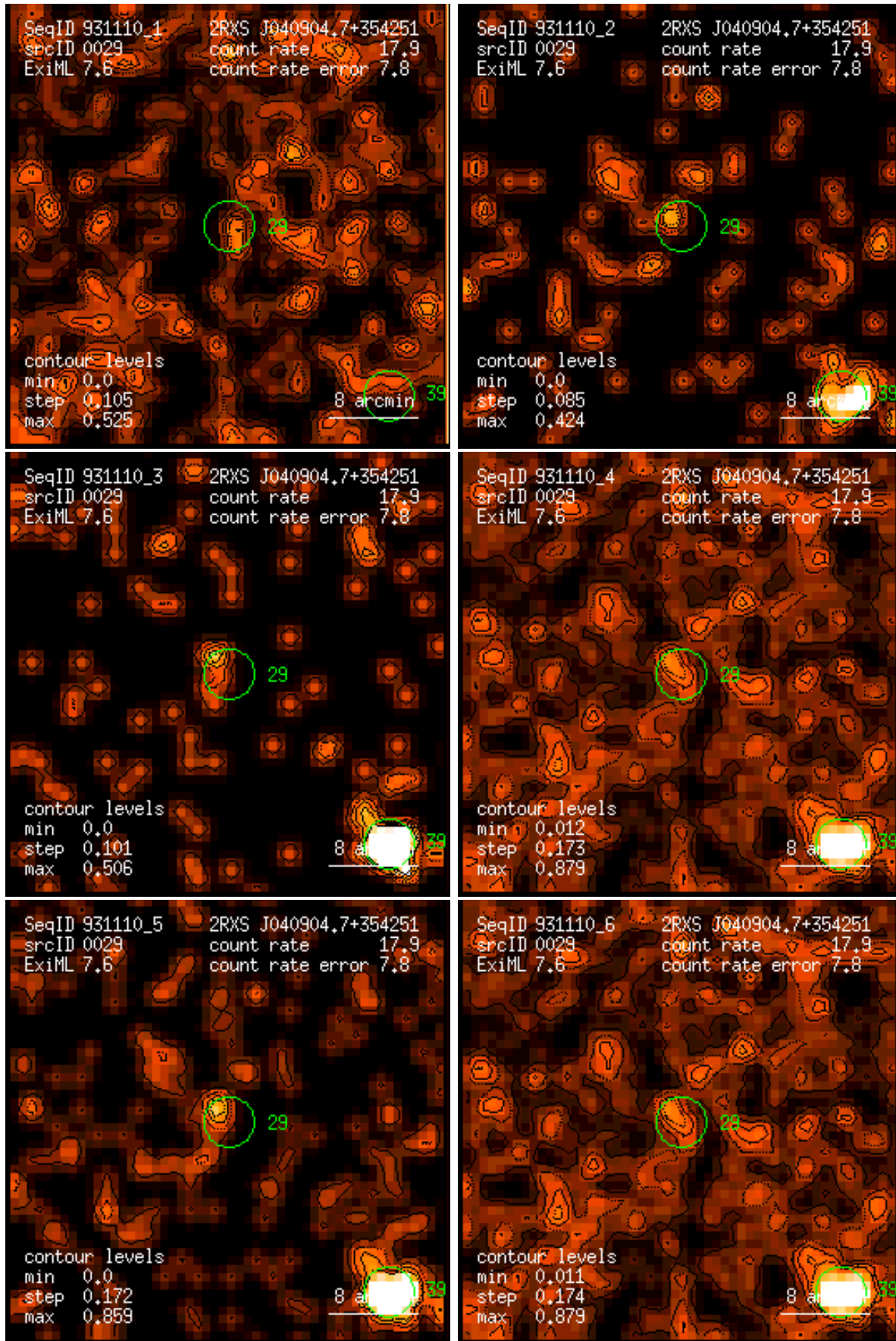
Figure 29: RASS 931110: detection 0029: band rate images, Gaussian filter: (1) PSPC channels 11 – 41, (2) 52 – 90, (3) 91 – 201, (4) 11 – 235, (5) 52 – 201, (6) 11 – 201. Broad band rates in counts/ks. Band rate contour levels in counts/ks/arcmin 2 .
