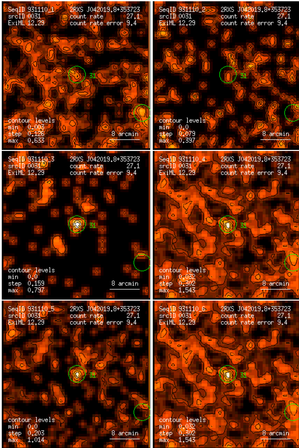
Figure 31: RASS 931110: detection 0031: band rate images, Gaussian filter: (1) PSPC channels 11 – 41, (2) 52 – 90, (3) 91 – 201, (4) 11 – 235, (5) 52 – 201, (6) 11 – 201. Broad band rates in counts/ks. Band rate contour levels in counts/ks/arcmin 2 .
