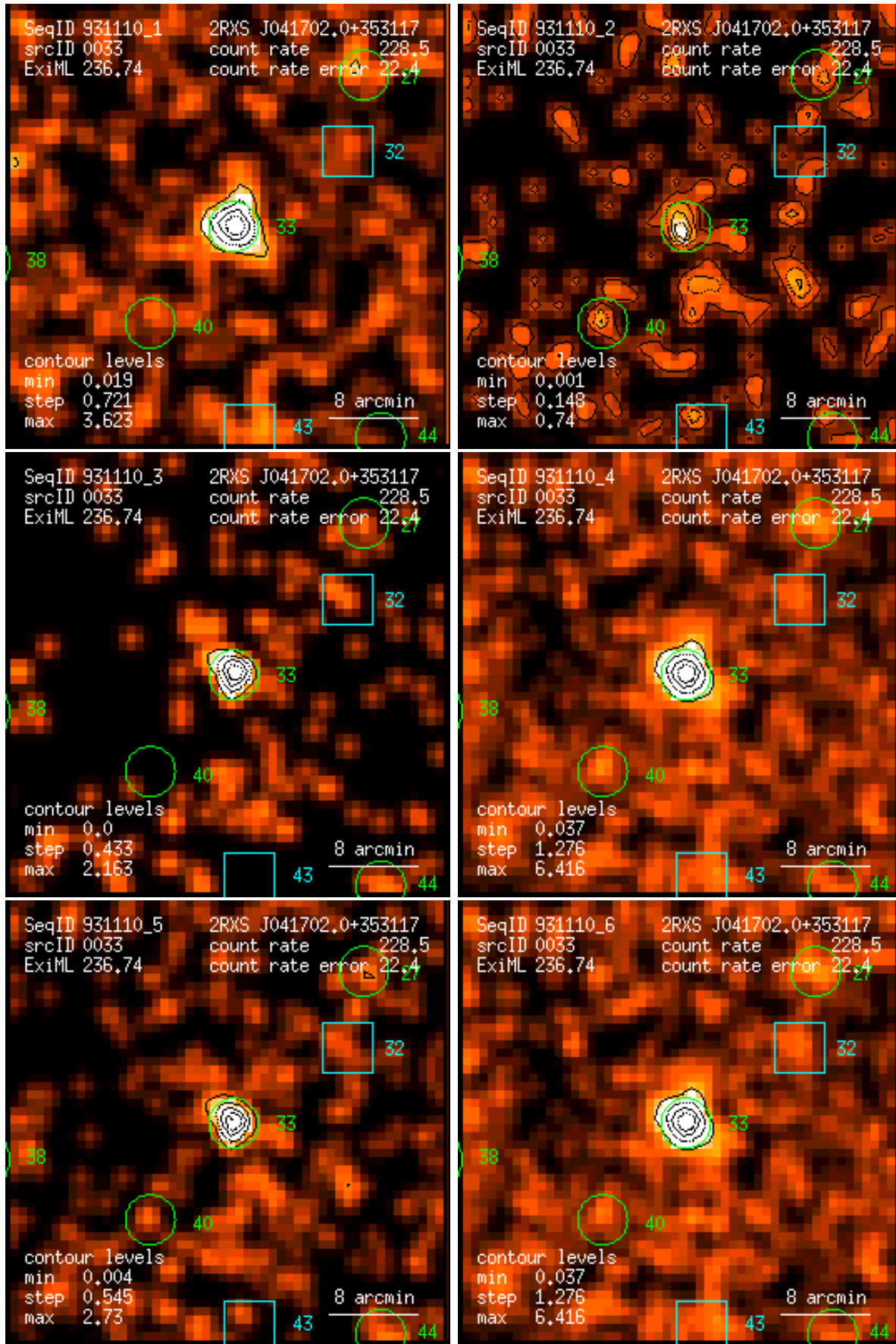
Figure 33: RASS 931110: detection 0033: band rate images, Gaussian filter: (1) PSPC channels 11 – 41, (2) 52 – 90, (3) 91 – 201, (4) 11 – 235, (5) 52 – 201, (6) 11 – 201. Broad band rates in counts/ks. Band rate contour levels in counts/ks/arcmin 2 .
