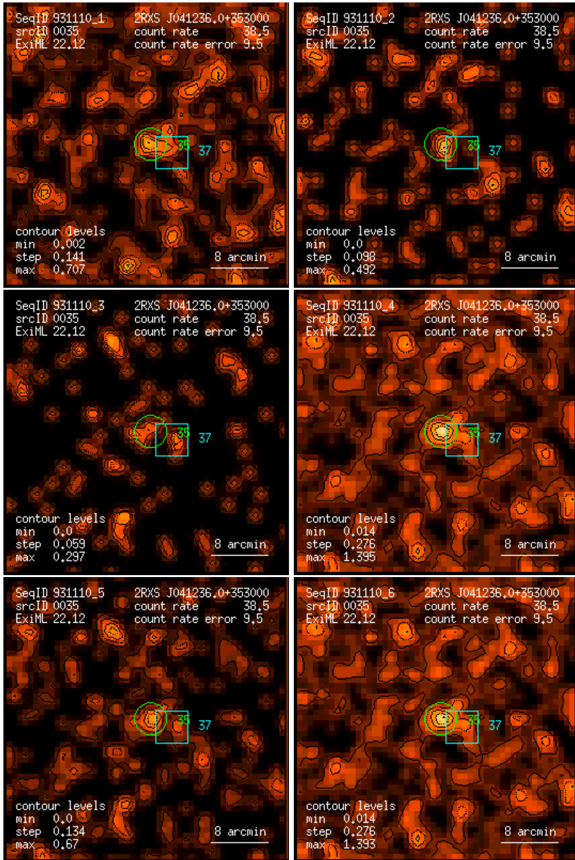
Figure 35: RASS 931110: detection 0035: band rate images, Gaussian filter: (1) PSPC channels 11 – 41, (2) 52 – 90, (3) 91 – 201, (4) 11 – 235, (5) 52 – 201, (6) 11 – 201. Broad band rates in counts/ks. Band rate contour levels in counts/ks/arcmin 2 .
