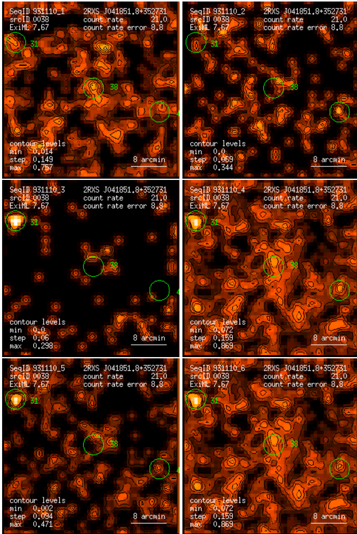
Figure 38: RASS 931110: detection 0038: band rate images, Gaussian filter: (1) PSPC channels 11 – 41, (2) 52 – 90, (3) 91 – 201, (4) 11 – 235, (5) 52 – 201, (6) 11 – 201. Broad band rates in counts/ks. Band rate contour levels in counts/ks/arcmin 2 .
