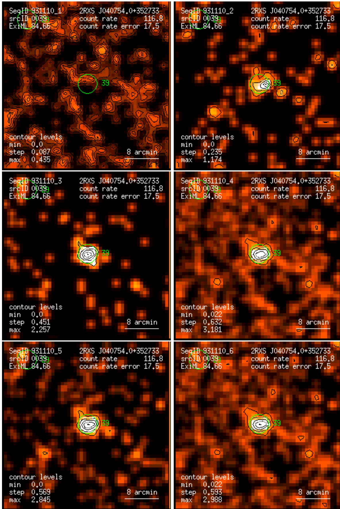
Figure 39: RASS 931110: detection 0039: band rate images, Gaussian filter: (1) PSPC channels 11 – 41, (2) 52 – 90, (3) 91 – 201, (4) 11 – 235, (5) 52 – 201, (6) 11 – 201. Broad band rates in counts/ks. Band rate contour levels in counts/ks/arcmin 2 .
