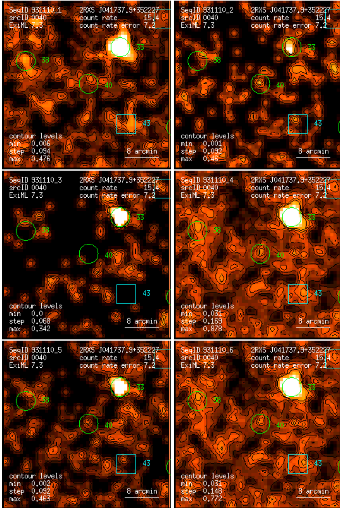
Figure 40: RASS 931110: detection 0040: band rate images, Gaussian filter: (1) PSPC channels 11 – 41, (2) 52 – 90, (3) 91 – 201, (4) 11 – 235, (5) 52 – 201, (6) 11 – 201. Broad band rates in counts/ks. Band rate contour levels in counts/ks/arcmin 2 .
