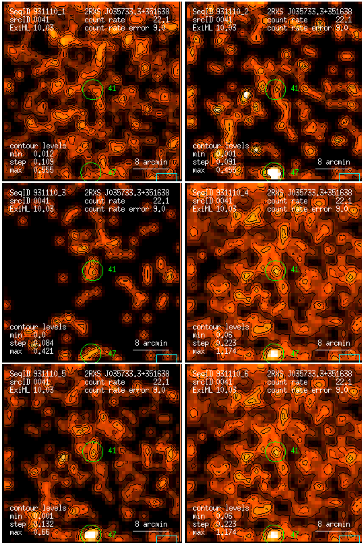
Figure 41: RASS 931110: detection 0041: band rate images, Gaussian filter: (1) PSPC channels 11 – 41, (2) 52 – 90, (3) 91 – 201, (4) 11 – 235, (5) 52 – 201, (6) 11 – 201. Broad band rates in counts/ks. Band rate contour levels in counts/ks/arcmin 2 .
