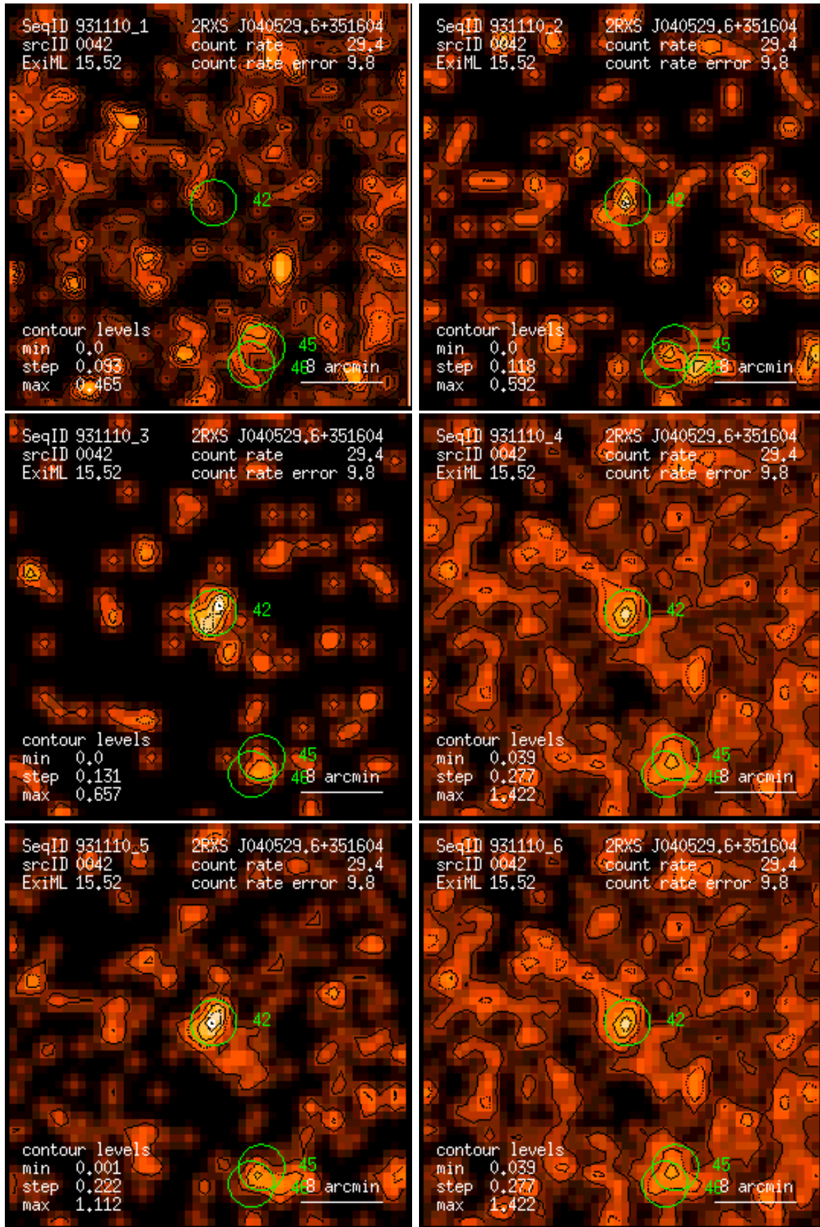
Figure 42: RASS 931110: detection 0042: band rate images, Gaussian filter: (1) PSPC channels 11 – 41, (2) 52 – 90, (3) 91 – 201, (4) 11 – 235, (5) 52 – 201, (6) 11 – 201. Broad band rates in counts/ks. Band rate contour levels in counts/ks/arcmin 2 .
