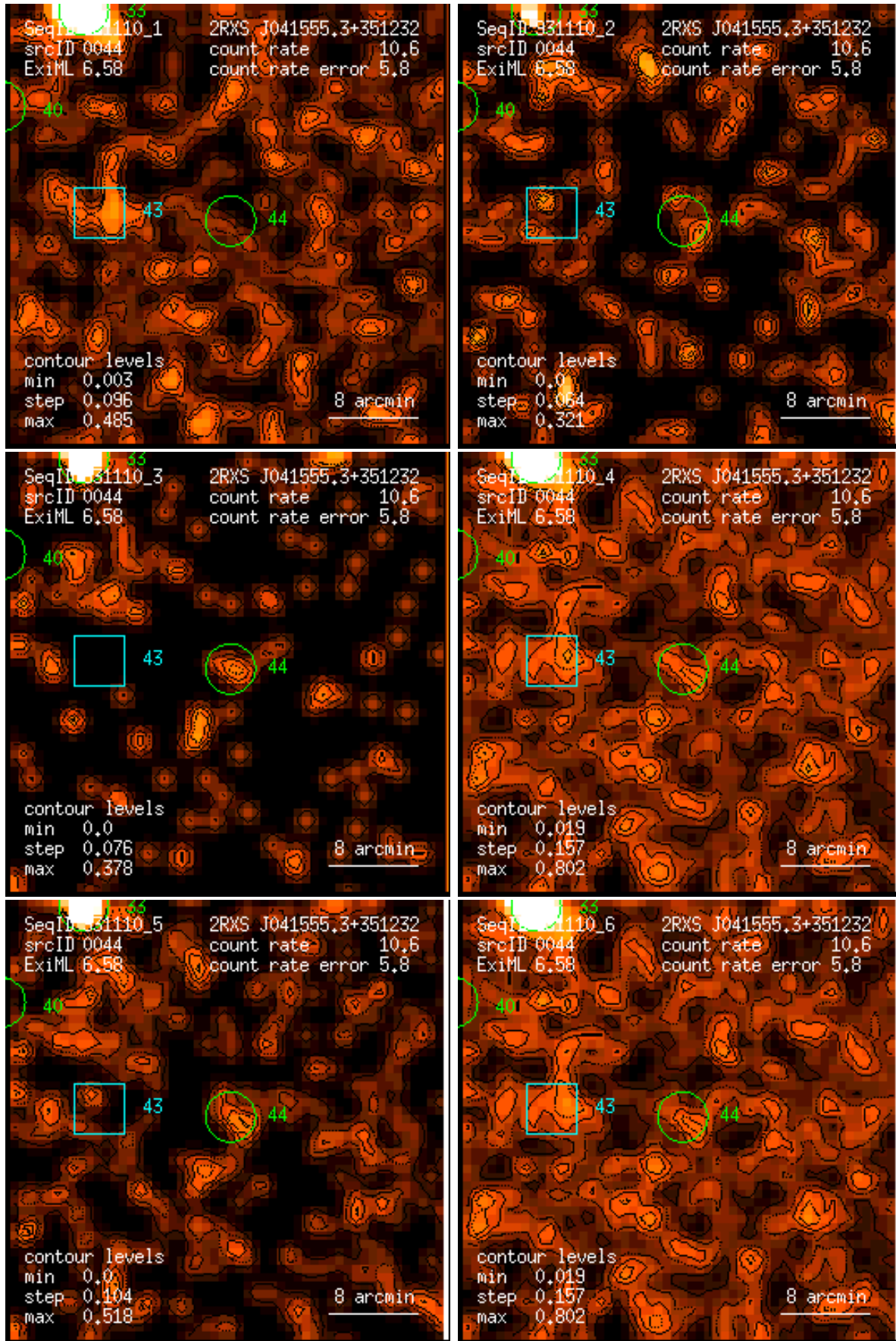
Figure 44: RASS 931110: detection 0044: band rate images, Gaussian filter: (1) PSPC channels 11 – 41, (2) 52 – 90, (3) 91 – 201, (4) 11 – 235, (5) 52 – 201, (6) 11 – 201. Broad band rates in counts/ks. Band rate contour levels in counts/ks/arcmin 2 .
