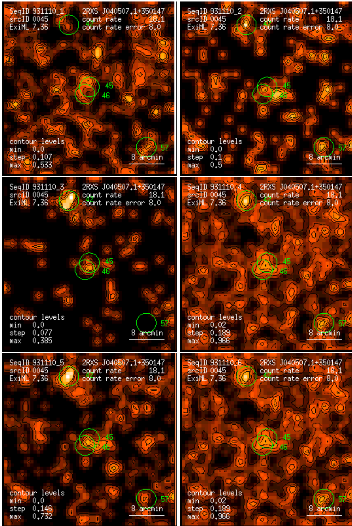
Figure 45: RASS 931110: detection 0045: band rate images, Gaussian filter: (1) PSPC channels 11 – 41, (2) 52 – 90, (3) 91 – 201, (4) 11 – 235, (5) 52 – 201, (6) 11 – 201. Broad band rates in counts/ks. Band rate contour levels in counts/ks/arcmin 2 .
