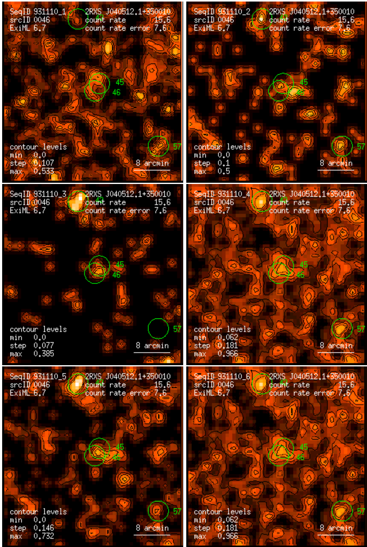
Figure 46: RASS 931110: detection 0046: band rate images, Gaussian filter: (1) PSPC channels 11 – 41, (2) 52 – 90, (3) 91 – 201, (4) 11 – 235, (5) 52 – 201, (6) 11 – 201. Broad band rates in counts/ks. Band rate contour levels in counts/ks/arcmin 2 .
