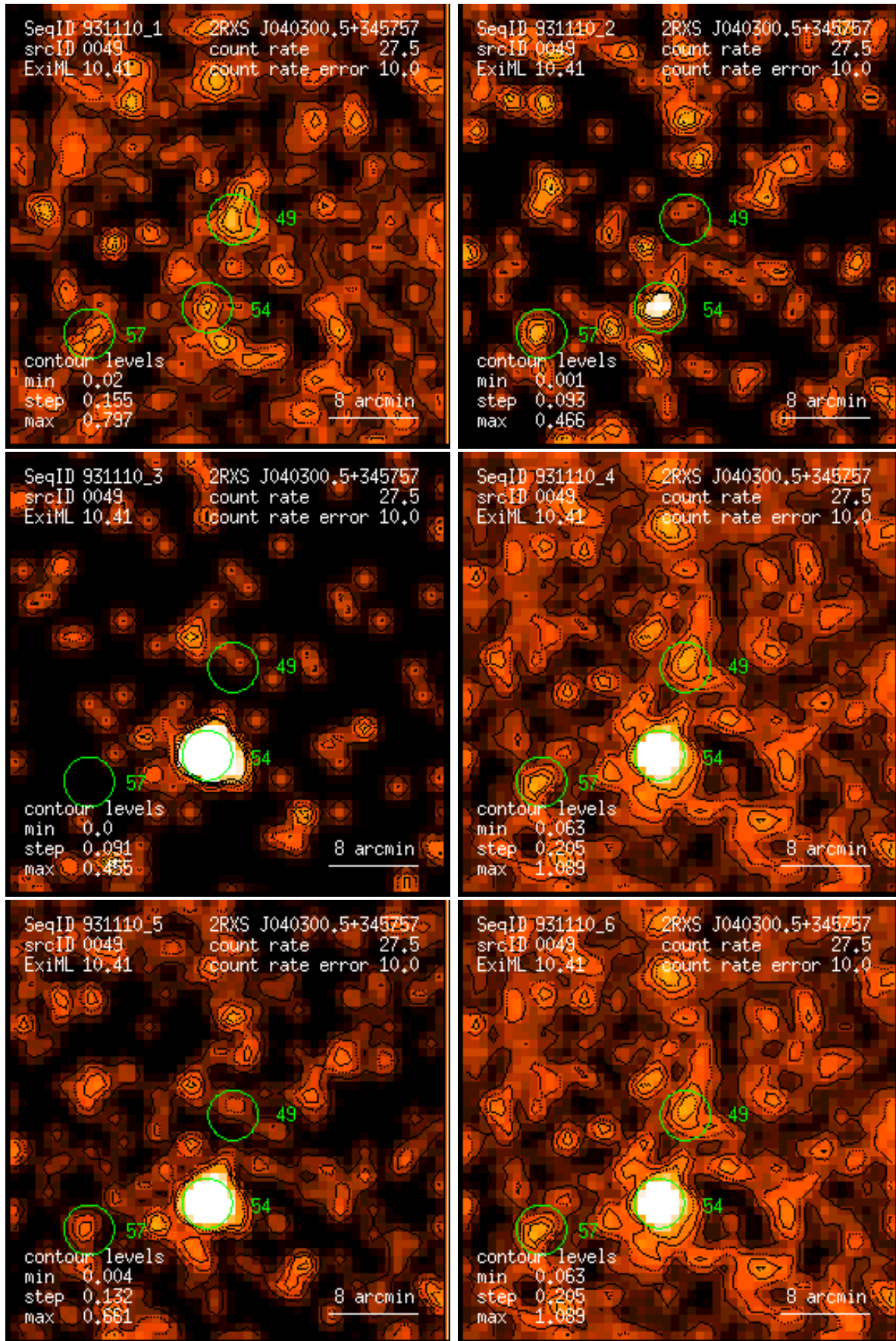
Figure 49: RASS 931110: detection 0049: band rate images, Gaussian filter: (1) PSPC channels 11 – 41, (2) 52 – 90, (3) 91 – 201, (4) 11 – 235, (5) 52 – 201, (6) 11 – 201. Broad band rates in counts/ks. Band rate contour levels in counts/ks/arcmin 2 .
