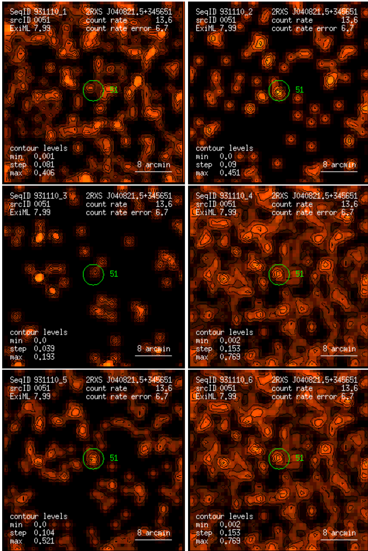
Figure 51: RASS 931110: detection 0051: band rate images, Gaussian filter: (1) PSPC channels 11 – 41, (2) 52 – 90, (3) 91 – 201, (4) 11 – 235, (5) 52 – 201, (6) 11 – 201. Broad band rates in counts/ks. Band rate contour levels in counts/ks/arcmin 2 .
