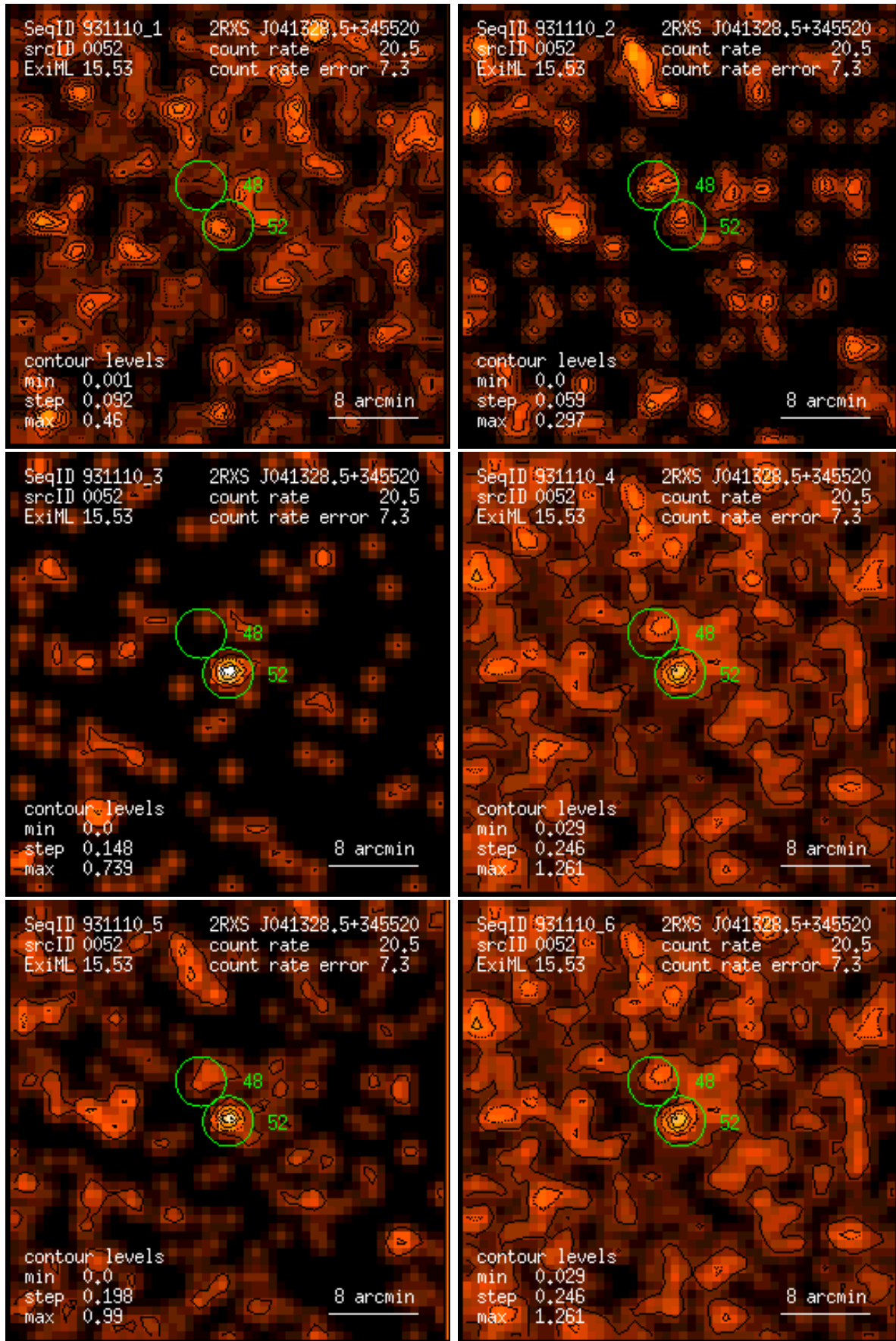
Figure 52: RASS 931110: detection 0052: band rate images, Gaussian filter: (1) PSPC channels 11 – 41, (2) 52 – 90, (3) 91 – 201, (4) 11 – 235, (5) 52 – 201, (6) 11 – 201. Broad band rates in counts/ks. Band rate contour levels in counts/ks/arcmin 2 .
