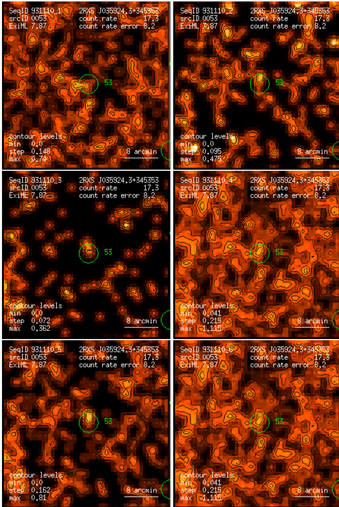
Figure 53: RASS 931110: detection 0053: band rate images, Gaussian filter: (1) PSPC channels 11 – 41, (2) 52 – 90, (3) 91 – 201, (4) 11 – 235, (5) 52 – 201, (6) 11 – 201. Broad band rates in counts/ks. Band rate contour levels in counts/ks/arcmin 2 .
