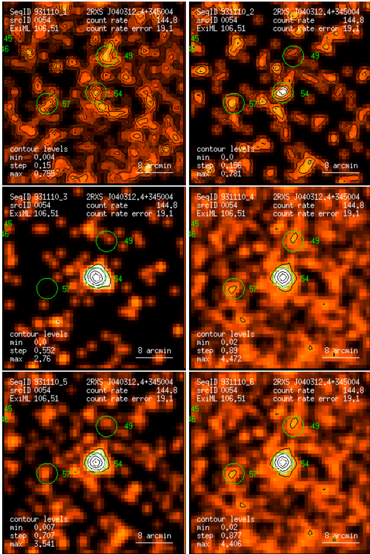
Figure 54: RASS 931110: detection 0054: band rate images, Gaussian filter: (1) PSPC channels 11 – 41, (2) 52 – 90, (3) 91 – 201, (4) 11 – 235, (5) 52 – 201, (6) 11 – 201. Broad band rates in counts/ks. Band rate contour levels in counts/ks/arcmin 2 .
