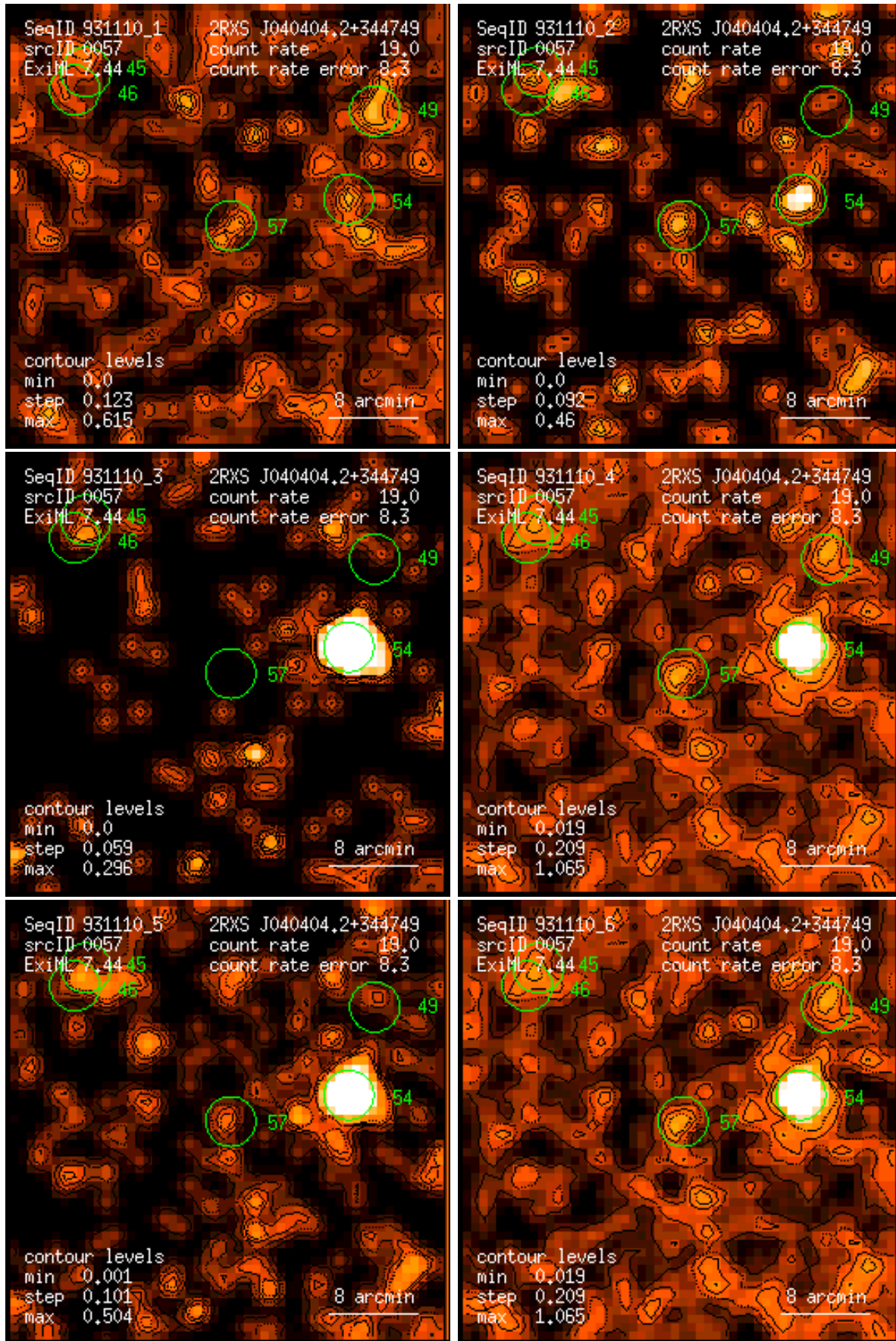
Figure 57: RASS 931110: detection 0057: band rate images, Gaussian filter: (1) PSPC channels 11 – 41, (2) 52 – 90, (3) 91 – 201, (4) 11 – 235, (5) 52 – 201, (6) 11 – 201. Broad band rates in counts/ks. Band rate contour levels in counts/ks/arcmin 2 .
