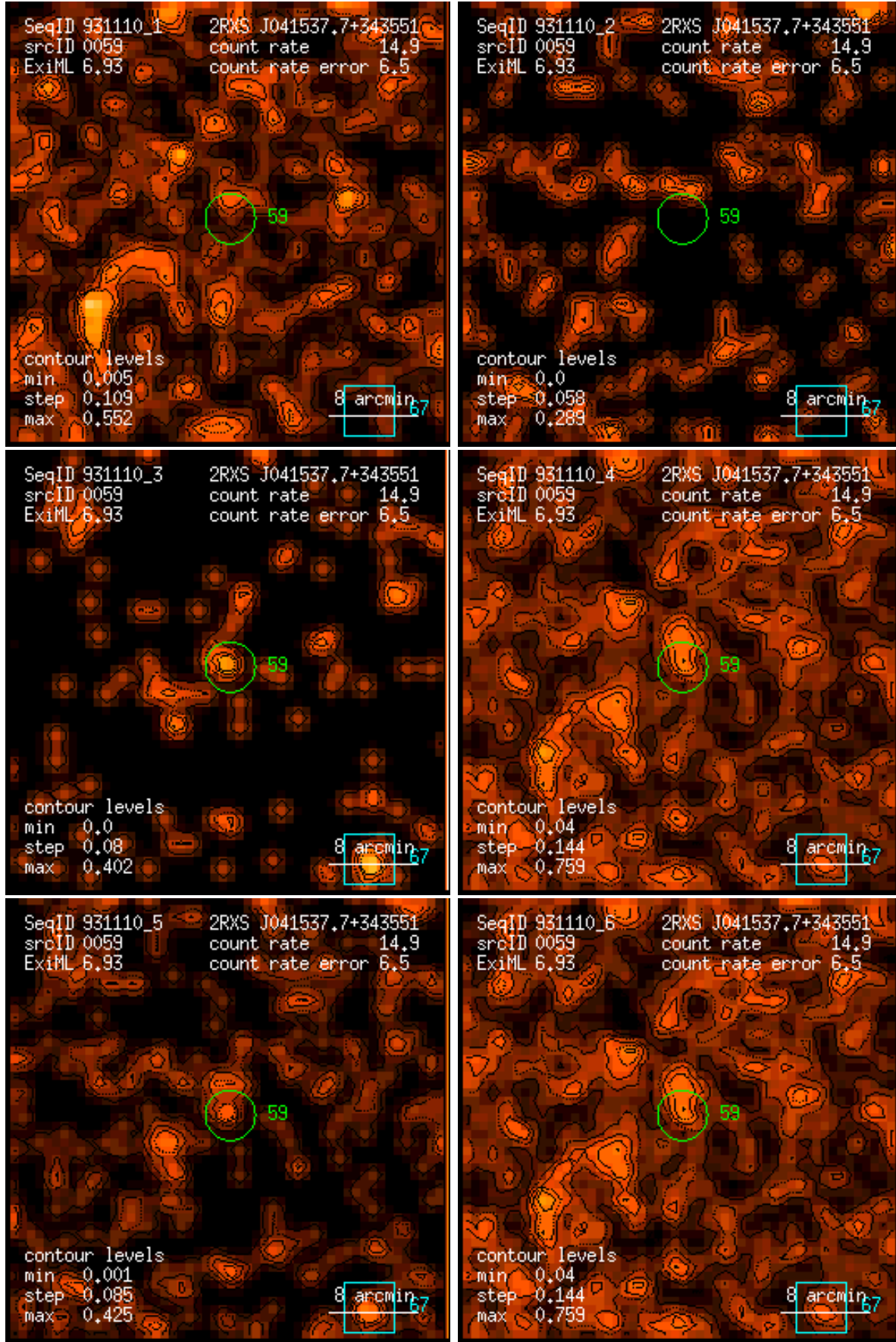
Figure 59: RASS 931110: detection 0059: band rate images, Gaussian filter: (1) PSPC channels 11 – 41, (2) 52 – 90, (3) 91 – 201, (4) 11 – 235, (5) 52 – 201, (6) 11 – 201. Broad band rates in counts/ks. Band rate contour levels in counts/ks/arcmin 2 .
