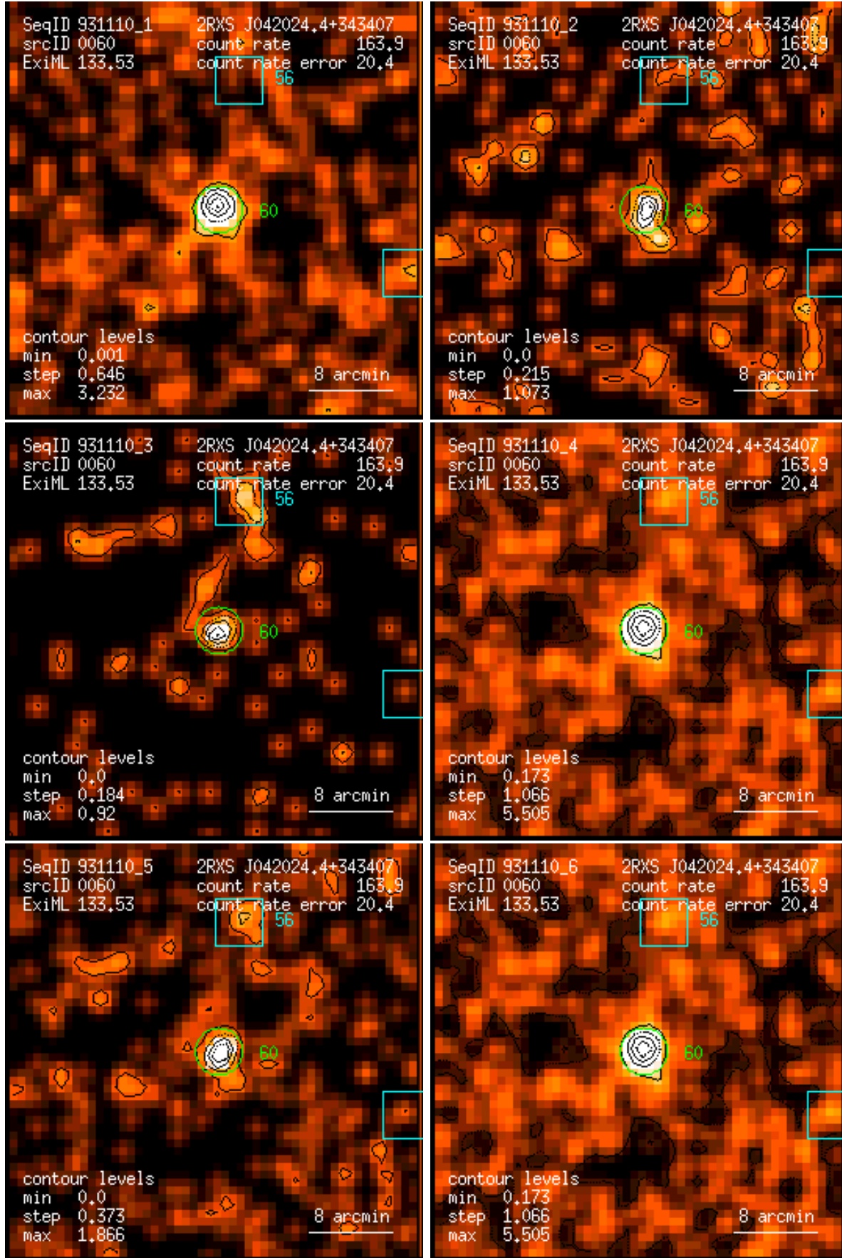
Figure 60: RASS 931110: detection 0060: band rate images, Gaussian filter: (1) PSPC channels 11 – 41, (2) 52 – 90, (3) 91 – 201, (4) 11 – 235, (5) 52 – 201, (6) 11 – 201. Broad band rates in counts/ks. Band rate contour levels in counts/ks/arcmin 2 .
