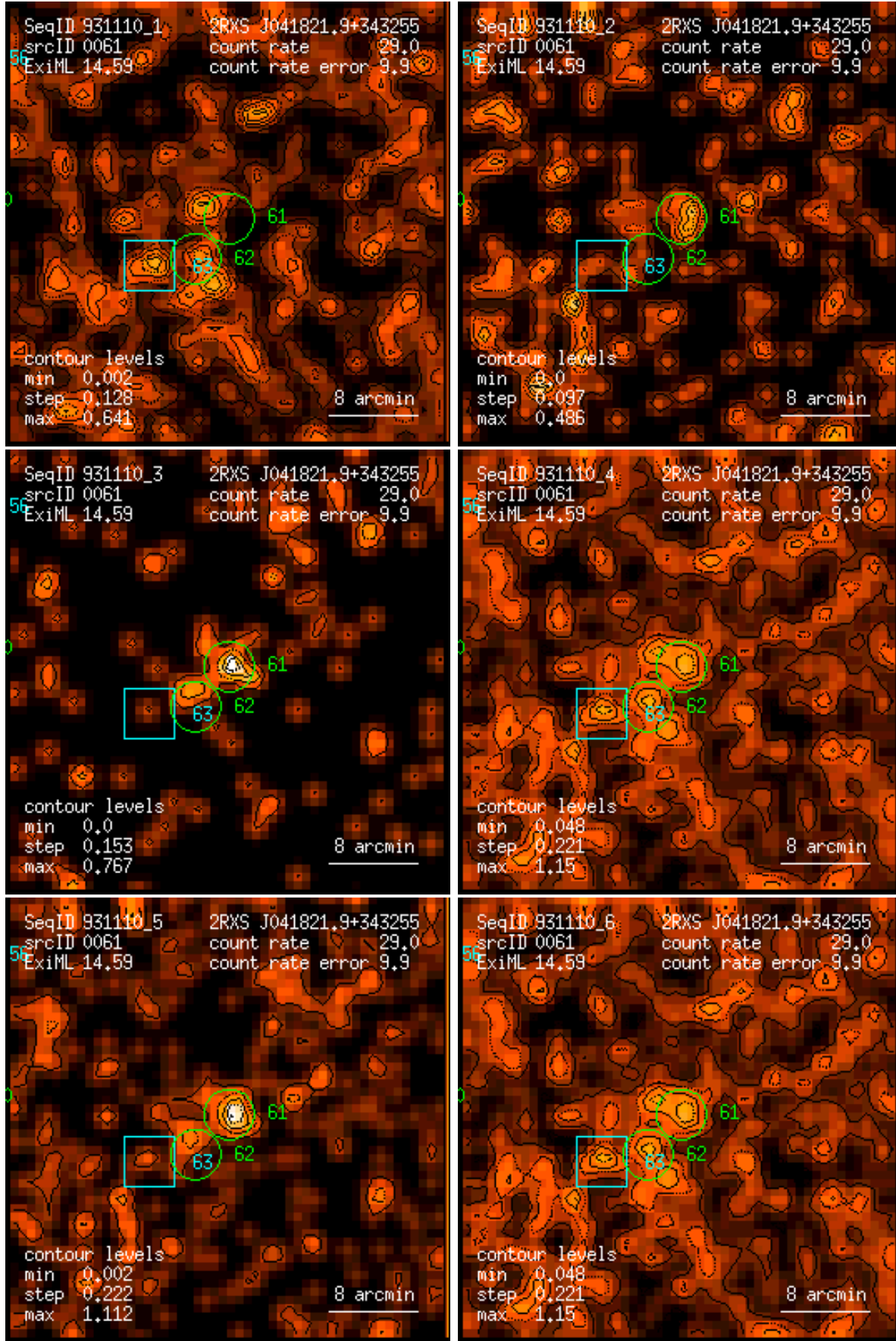
Figure 61: RASS 931110: detection 0061: band rate images, Gaussian filter: (1) PSPC channels 11 – 41, (2) 52 – 90, (3) 91 – 201, (4) 11 – 235, (5) 52 – 201, (6) 11 – 201. Broad band rates in counts/ks. Band rate contour levels in counts/ks/arcmin 2 .
