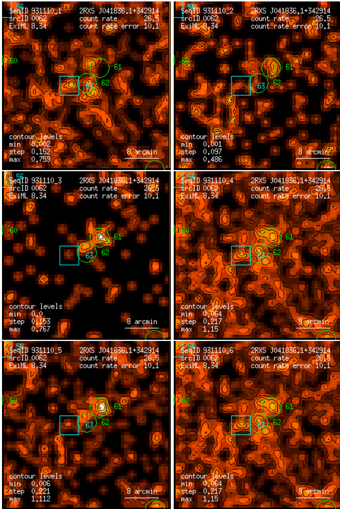
Figure 62: RASS 931110: detection 0062: band rate images, Gaussian filter: (1) PSPC channels 11 – 41, (2) 52 – 90, (3) 91 – 201, (4) 11 – 235, (5) 52 – 201, (6) 11 – 201. Broad band rates in counts/ks. Band rate contour levels in counts/ks/arcmin 2 .
