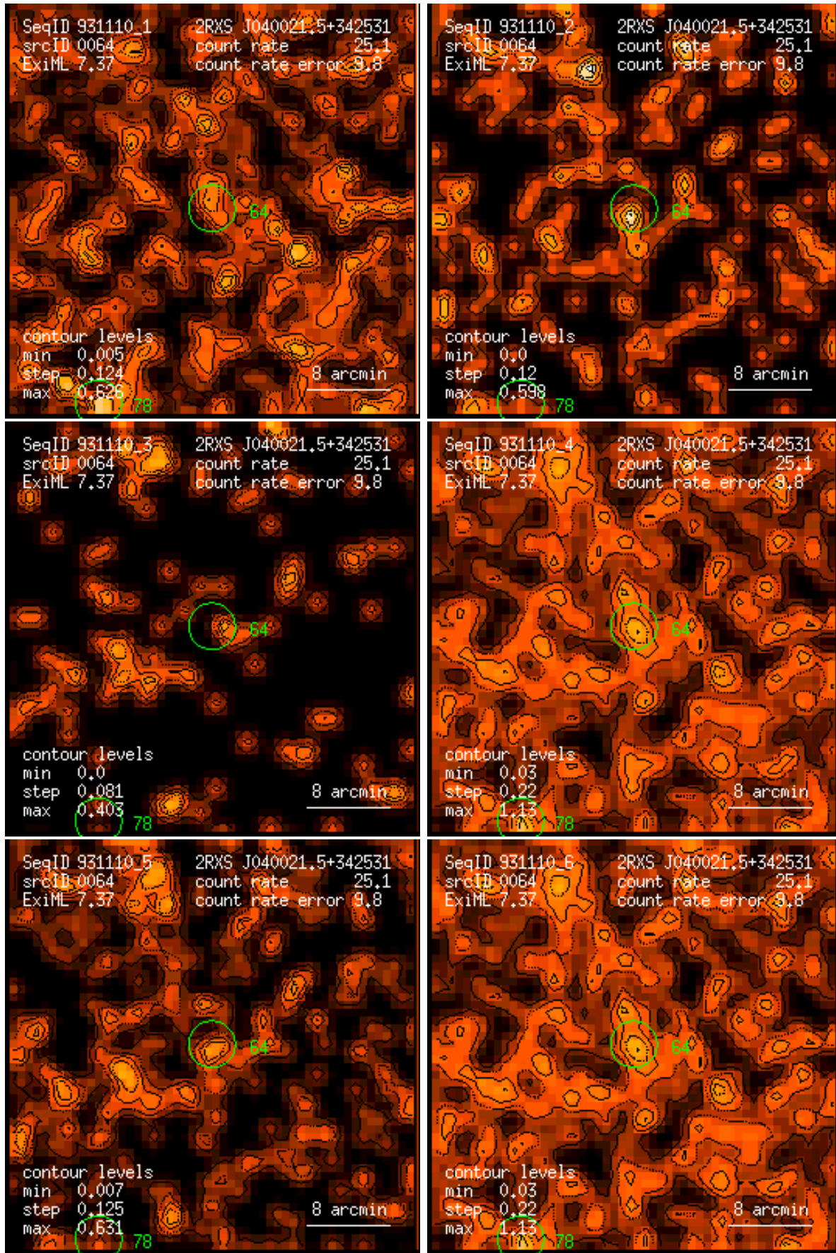
Figure 64: RASS 931110: detection 0064: band rate images, Gaussian filter: (1) PSPC channels 11 – 41, (2) 52 – 90, (3) 91 – 201, (4) 11 – 235, (5) 52 – 201, (6) 11 – 201. Broad band rates in counts/ks. Band rate contour levels in counts/ks/arcmin 2 .
