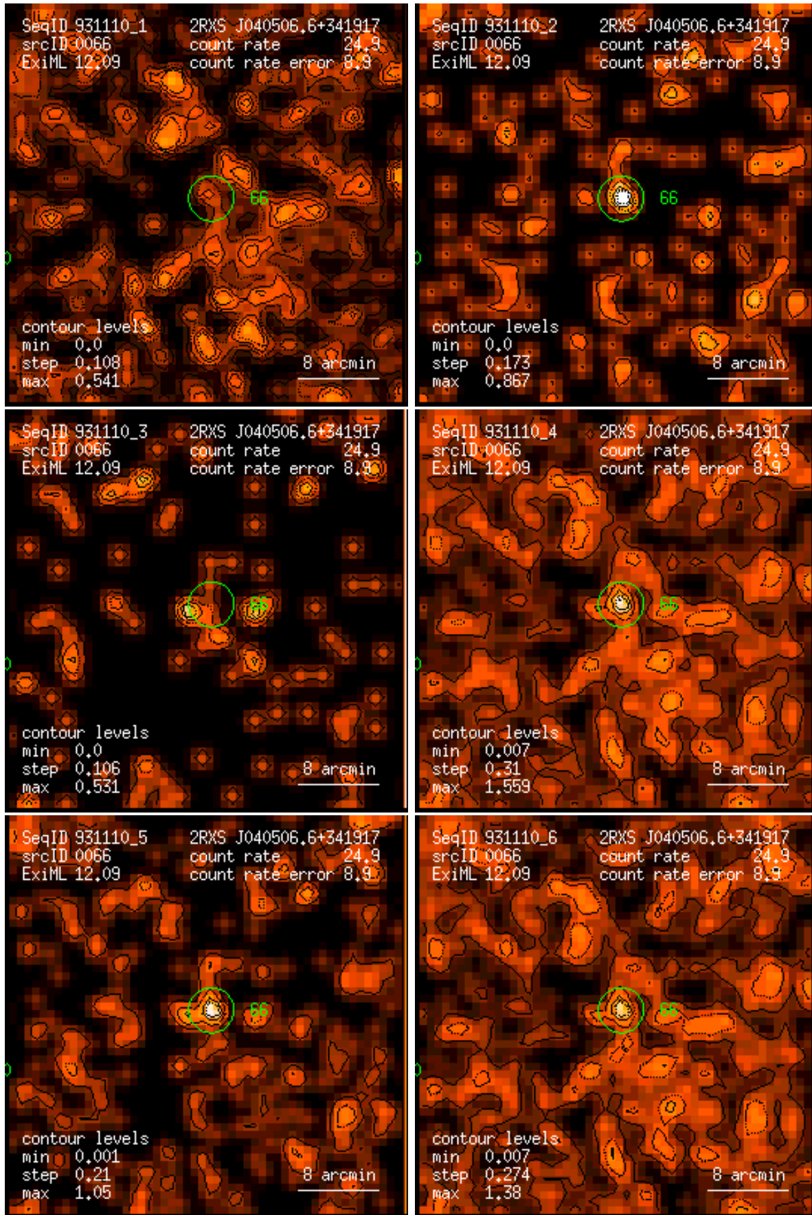
Figure 66: RASS 931110: detection 0066: band rate images, Gaussian filter: (1) PSPC channels 11 – 41, (2) 52 – 90, (3) 91 – 201, (4) 11 – 235, (5) 52 – 201, (6) 11 – 201. Broad band rates in counts/ks. Band rate contour levels in counts/ks/arcmin 2 .
