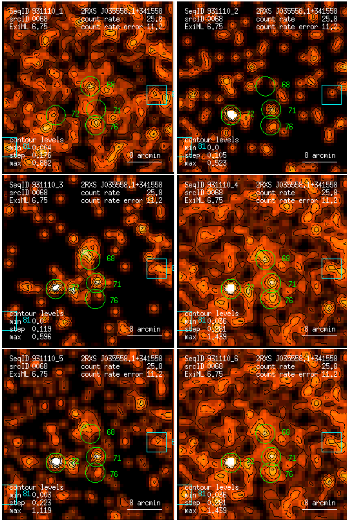
Figure 68: RASS 931110: detection 0068: band rate images, Gaussian filter: (1) PSPC channels 11 – 41, (2) 52 – 90, (3) 91 – 201, (4) 11 – 235, (5) 52 – 201, (6) 11 – 201. Broad band rates in counts/ks. Band rate contour levels in counts/ks/arcmin 2 .
