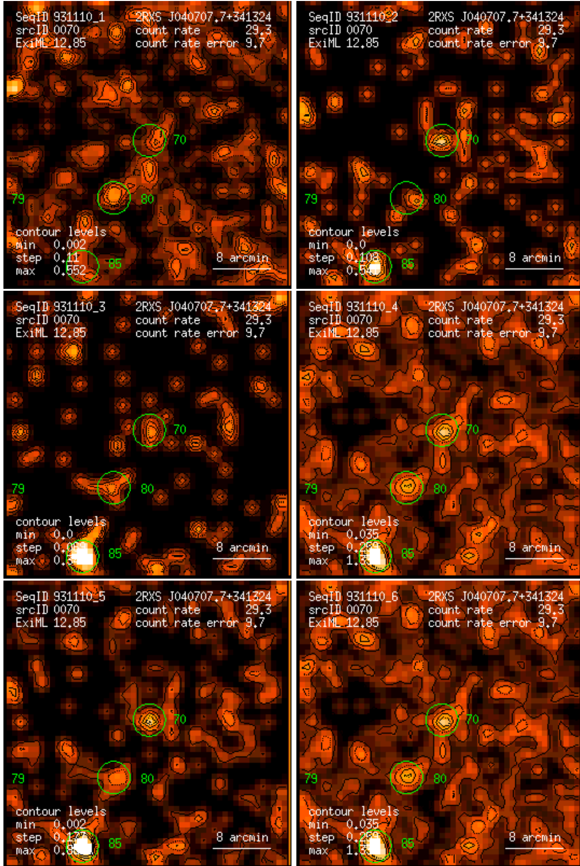
Figure 70: RASS 931110: detection 0070: band rate images, Gaussian filter: (1) PSPC channels 11 – 41, (2) 52 – 90, (3) 91 – 201, (4) 11 – 235, (5) 52 – 201, (6) 11 – 201. Broad band rates in counts/ks. Band rate contour levels in counts/ks/arcmin 2 .
