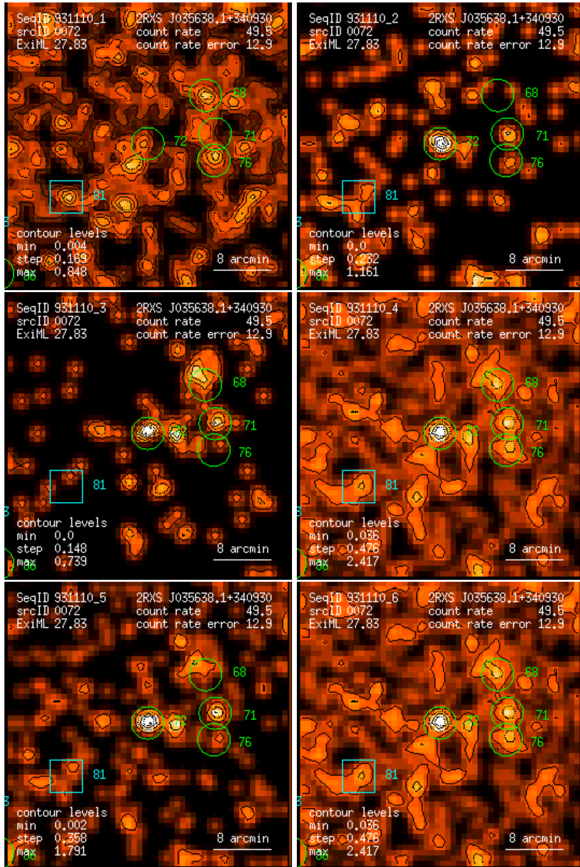
Figure 72: RASS 931110: detection 0072: band rate images, Gaussian filter: (1) PSPC channels 11 – 41, (2) 52 – 90, (3) 91 – 201, (4) 11 – 235, (5) 52 – 201, (6) 11 – 201. Broad band rates in counts/ks. Band rate contour levels in counts/ks/arcmin 2 .
