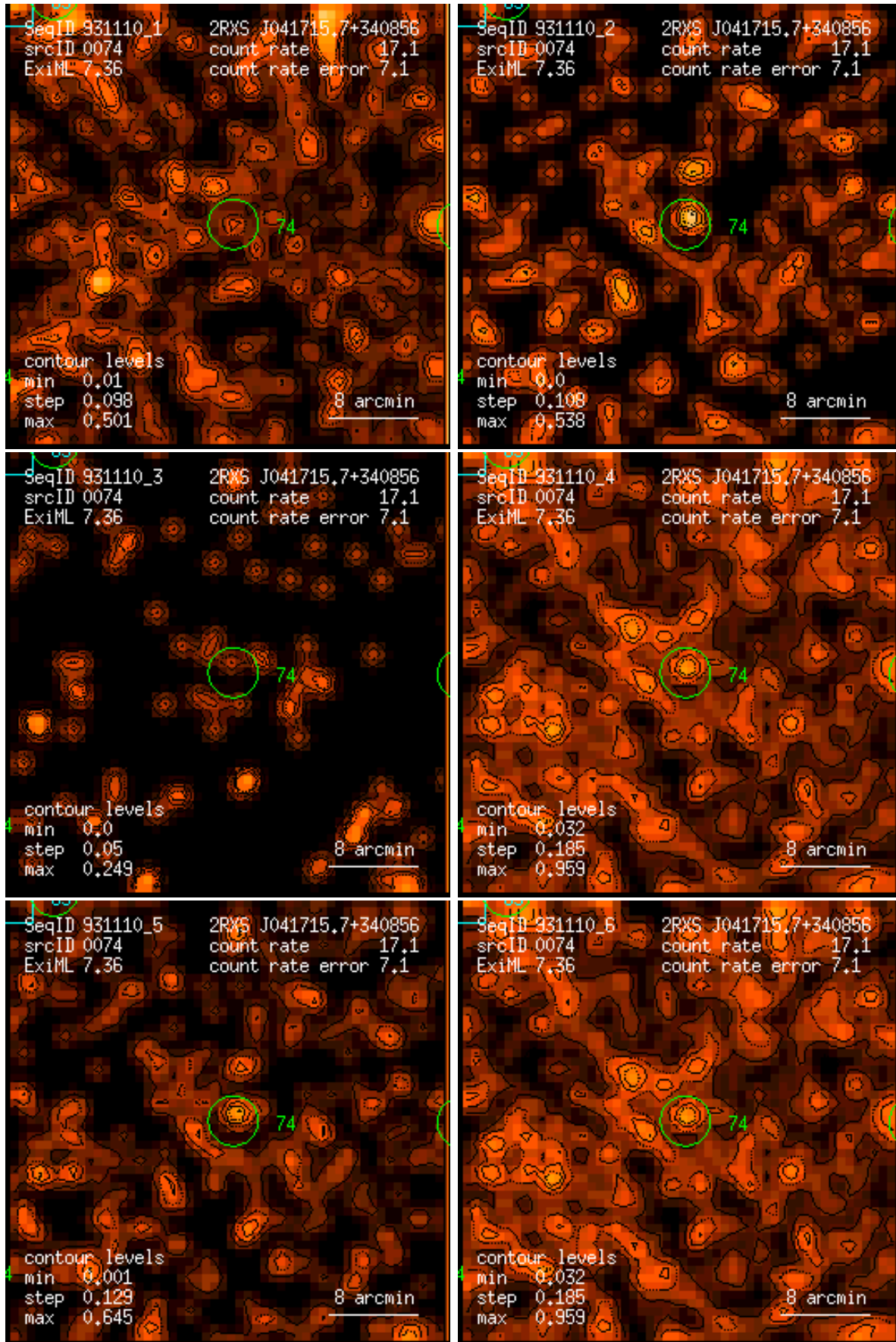
Figure 74: RASS 931110: detection 0074: band rate images, Gaussian filter: (1) PSPC channels 11 – 41, (2) 52 – 90, (3) 91 – 201, (4) 11 – 235, (5) 52 – 201, (6) 11 – 201. Broad band rates in counts/ks. Band rate contour levels in counts/ks/arcmin 2 .
