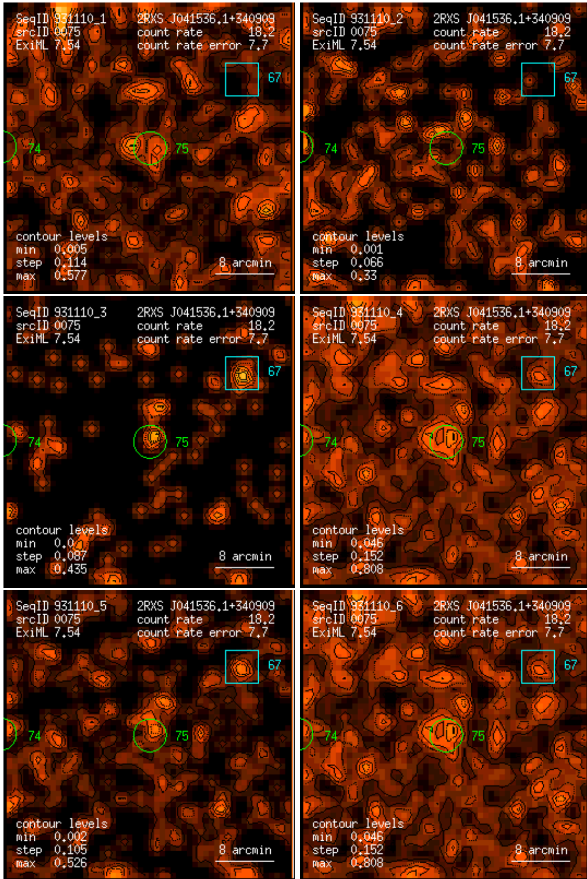
Figure 75: RASS 931110: detection 0075: band rate images, Gaussian filter: (1) PSPC channels 11 – 41, (2) 52 – 90, (3) 91 – 201, (4) 11 – 235, (5) 52 – 201, (6) 11 – 201. Broad band rates in counts/ks. Band rate contour levels in counts/ks/arcmin 2 .
