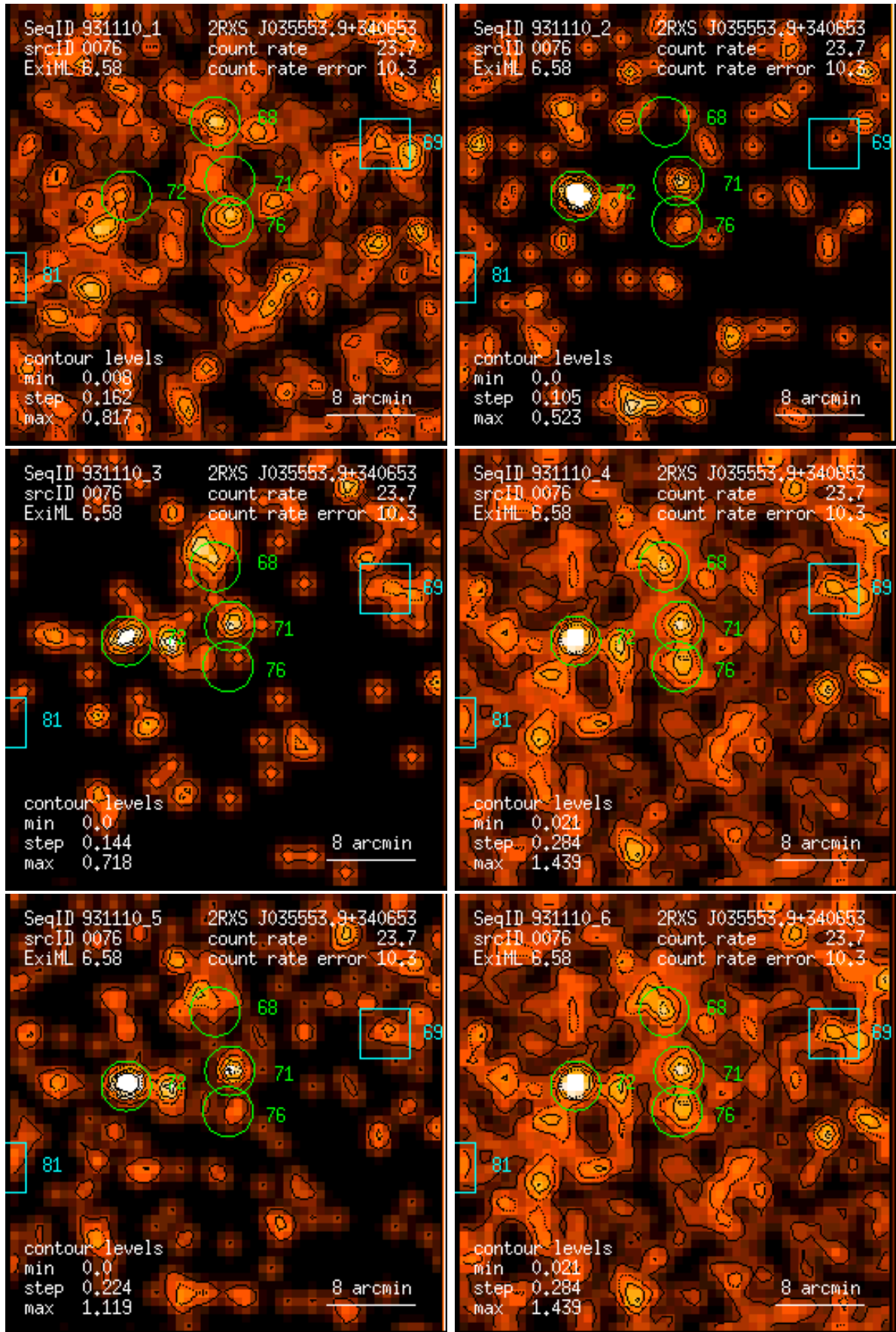
Figure 76: RASS 931110: detection 0076: band rate images, Gaussian filter: (1) PSPC channels 11 – 41, (2) 52 – 90, (3) 91 – 201, (4) 11 – 235, (5) 52 – 201, (6) 11 – 201. Broad band rates in counts/ks. Band rate contour levels in counts/ks/arcmin 2 .
