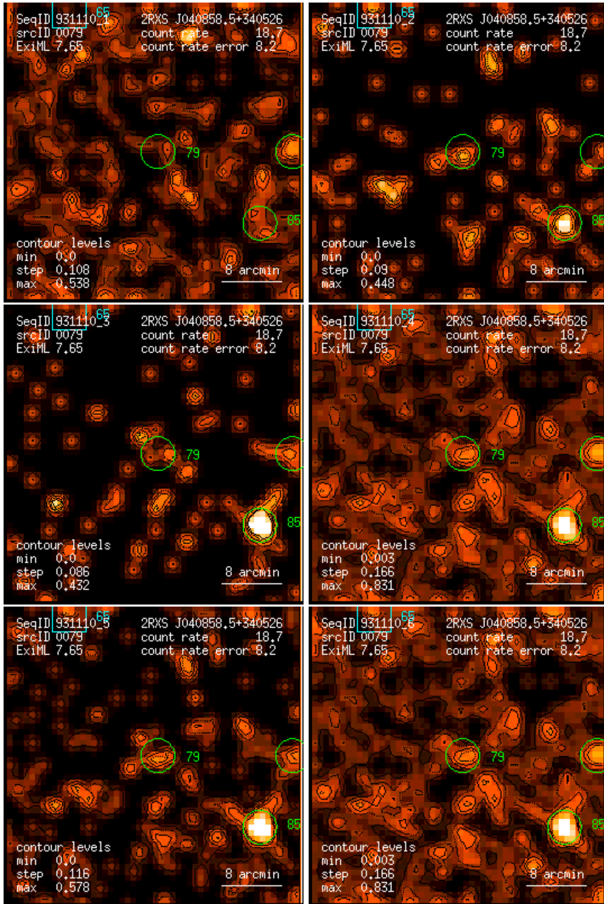
Figure 79: RASS 931110: detection 0079: band rate images, Gaussian filter: (1) PSPC channels 11 – 41, (2) 52 – 90, (3) 91 – 201, (4) 11 – 235, (5) 52 – 201, (6) 11 – 201. Broad band rates in counts/ks. Band rate contour levels in counts/ks/arcmin 2 .
