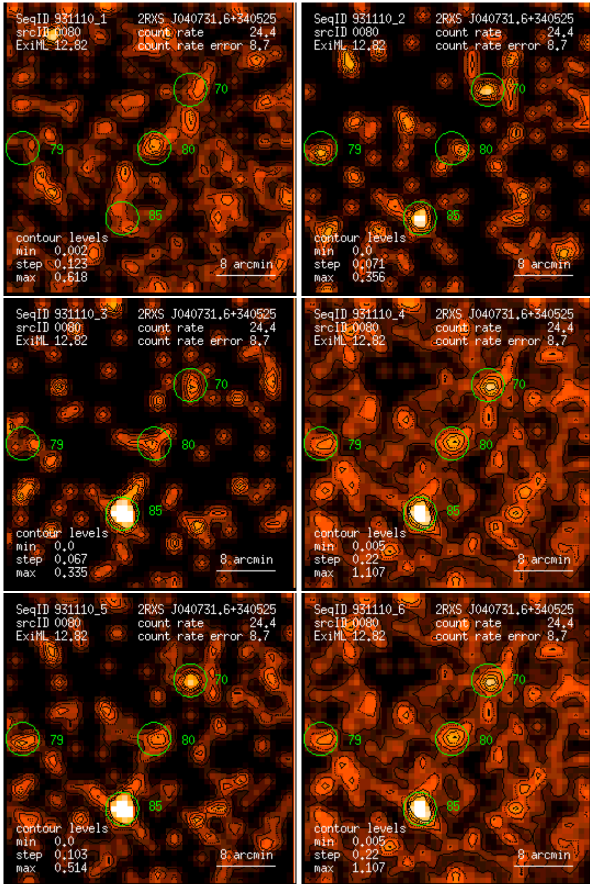
Figure 80: RASS 931110: detection 0080: band rate images, Gaussian filter: (1) PSPC channels 11 – 41, (2) 52 – 90, (3) 91 – 201, (4) 11 – 235, (5) 52 – 201, (6) 11 – 201. Broad band rates in counts/ks. Band rate contour levels in counts/ks/arcmin 2 .
