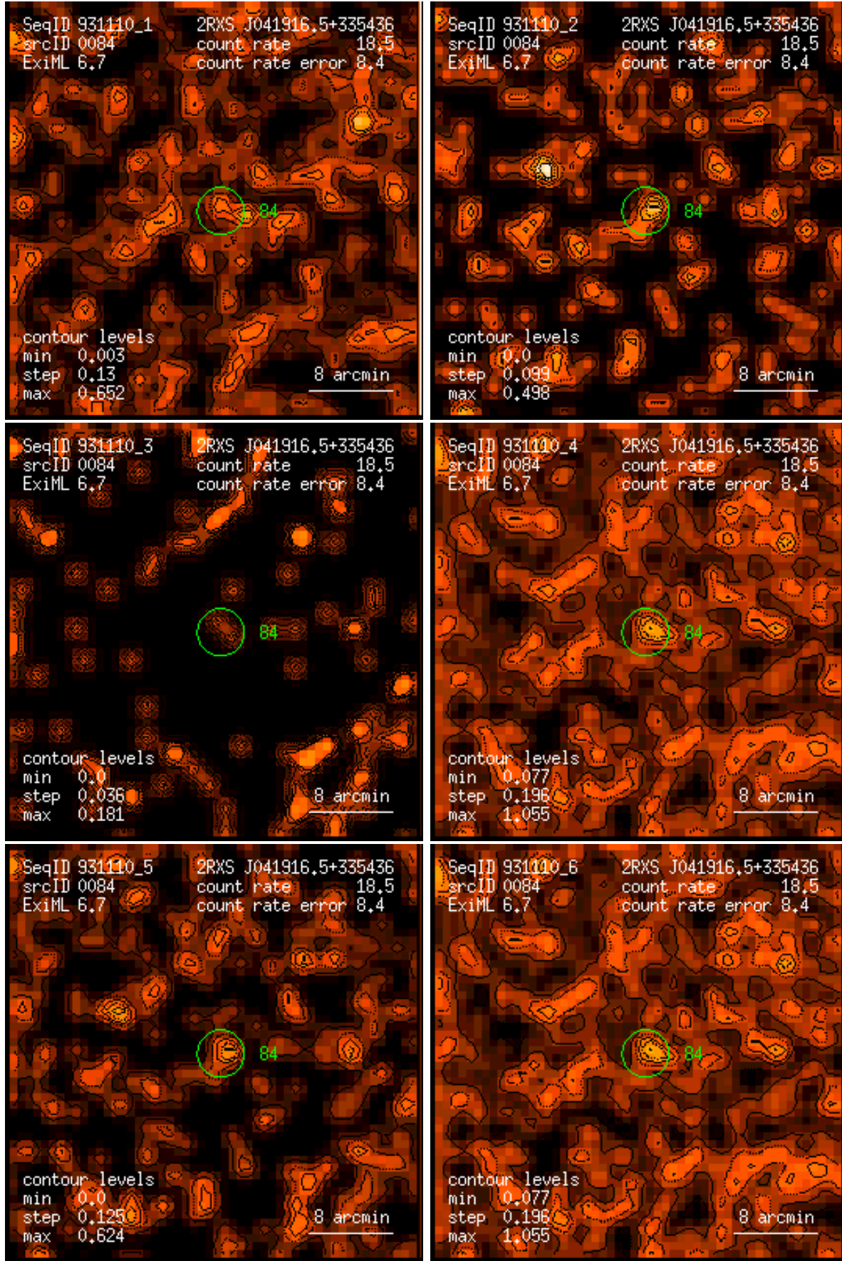
Figure 84: RASS 931110: detection 0084: band rate images, Gaussian filter: (1) PSPC channels 11 – 41, (2) 52 – 90, (3) 91 – 201, (4) 11 – 235, (5) 52 – 201, (6) 11 – 201. Broad band rates in counts/ks. Band rate contour levels in counts/ks/arcmin 2 .
