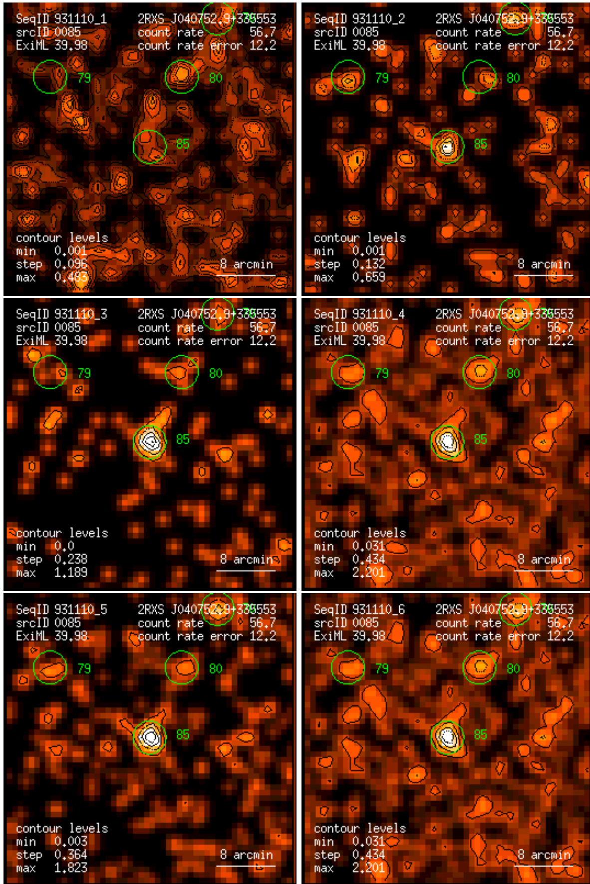
Figure 85: RASS 931110: detection 0085: band rate images, Gaussian filter: (1) PSPC channels 11 – 41, (2) 52 – 90, (3) 91 – 201, (4) 11 – 235, (5) 52 – 201, (6) 11 – 201. Broad band rates in counts/ks. Band rate contour levels in counts/ks/arcmin 2 .
