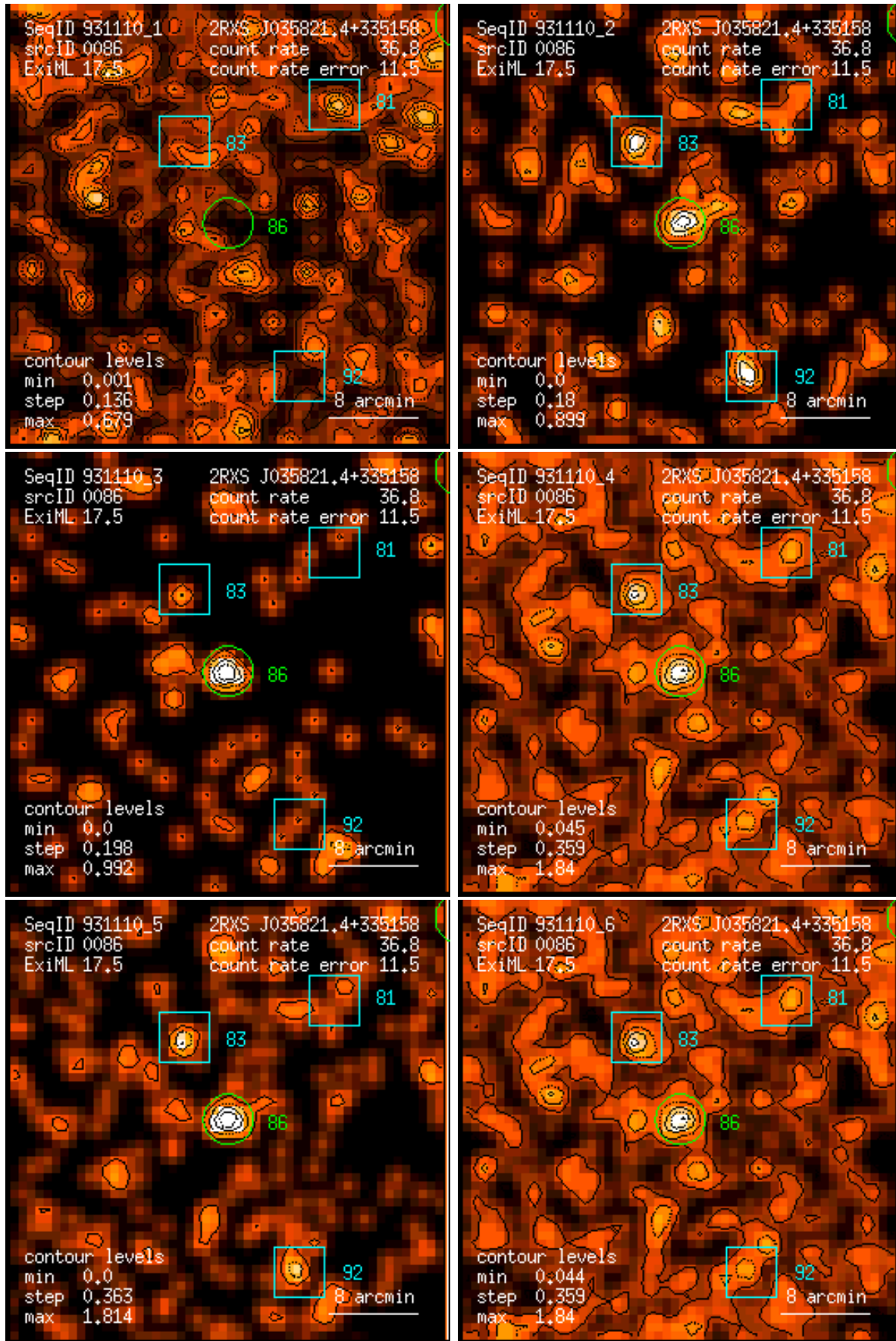
Figure 86: RASS 931110: detection 0086: band rate images, Gaussian filter: (1) PSPC channels 11 – 41, (2) 52 – 90, (3) 91 – 201, (4) 11 – 235, (5) 52 – 201, (6) 11 – 201. Broad band rates in counts/ks. Band rate contour levels in counts/ks/arcmin 2 .
