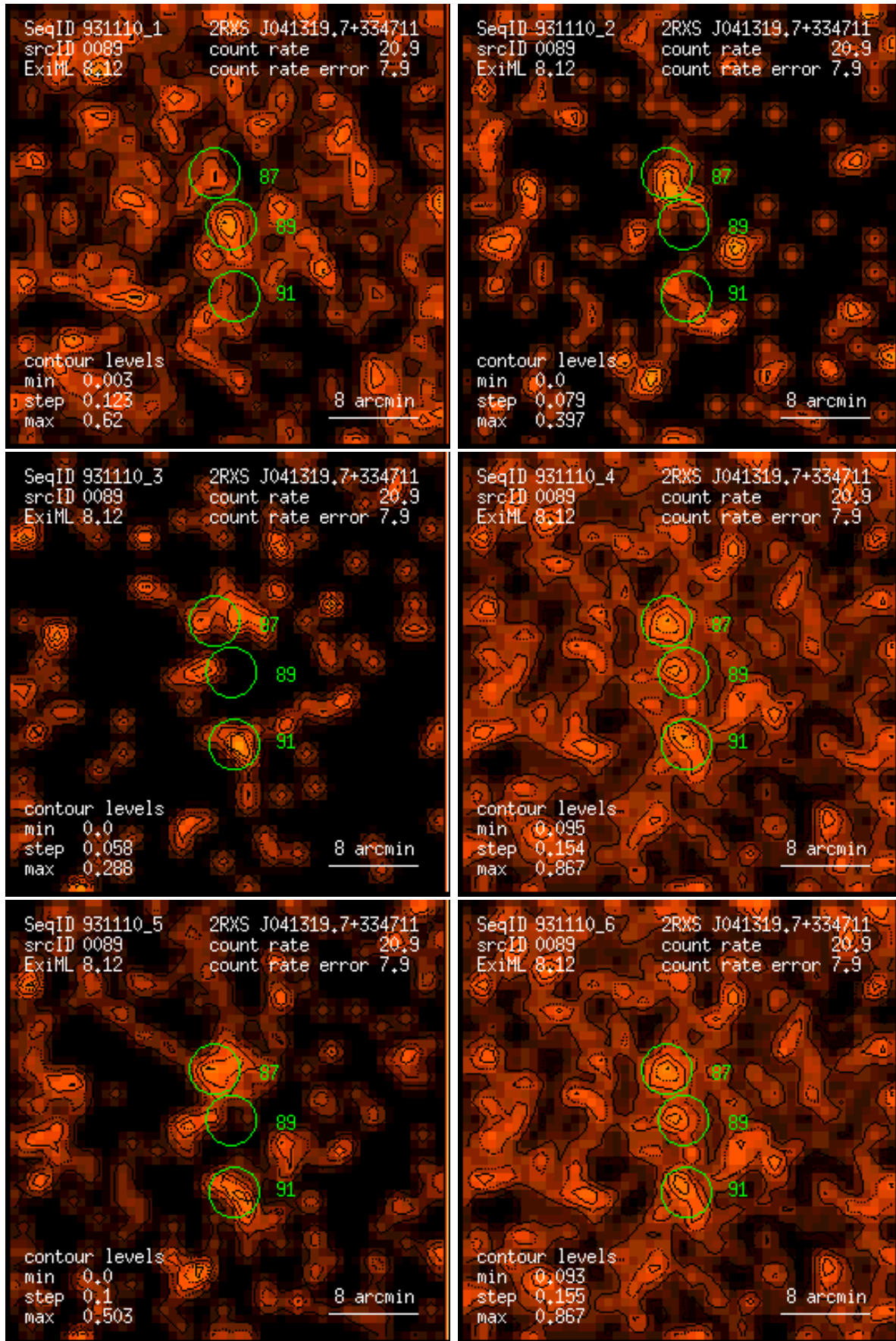
Figure 89: RASS 931110: detection 0089: band rate images, Gaussian filter: (1) PSPC channels 11 – 41, (2) 52 – 90, (3) 91 – 201, (4) 11 – 235, (5) 52 – 201, (6) 11 – 201. Broad band rates in counts/ks. Band rate contour levels in counts/ks/arcmin 2 .
