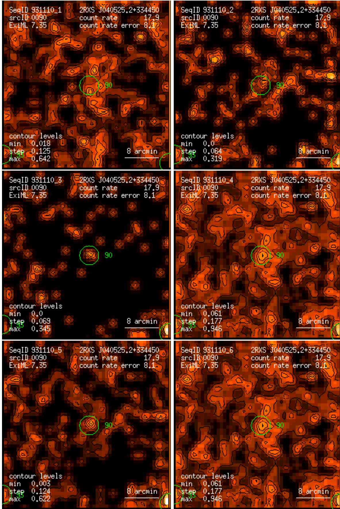
Figure 90: RASS 931110: detection 0090: band rate images, Gaussian filter: (1) PSPC channels 11 – 41, (2) 52 – 90, (3) 91 – 201, (4) 11 – 235, (5) 52 – 201, (6) 11 – 201. Broad band rates in counts/ks. Band rate contour levels in counts/ks/arcmin 2 .
