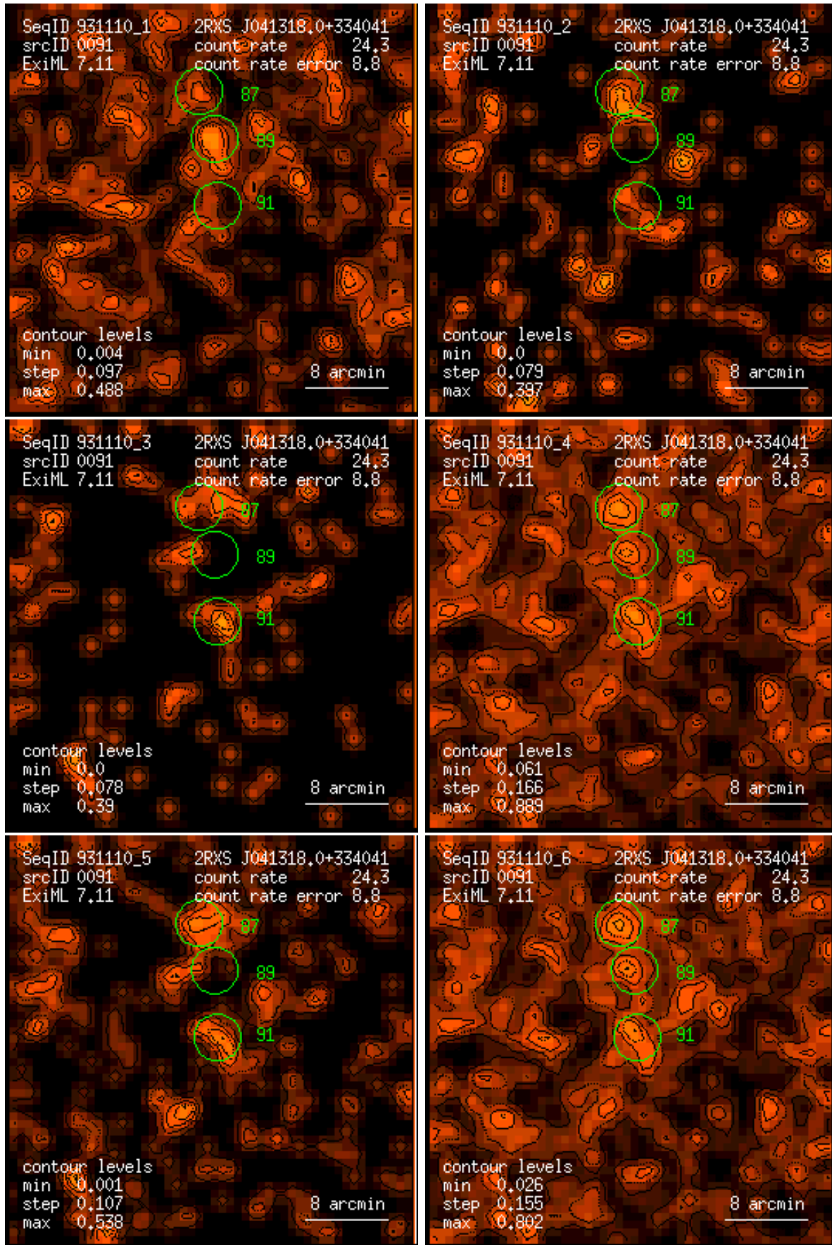
Figure 91: RASS 931110: detection 0091: band rate images, Gaussian filter: (1) PSPC channels 11 – 41, (2) 52 – 90, (3) 91 – 201, (4) 11 – 235, (5) 52 – 201, (6) 11 – 201. Broad band rates in counts/ks. Band rate contour levels in counts/ks/arcmin 2 .
