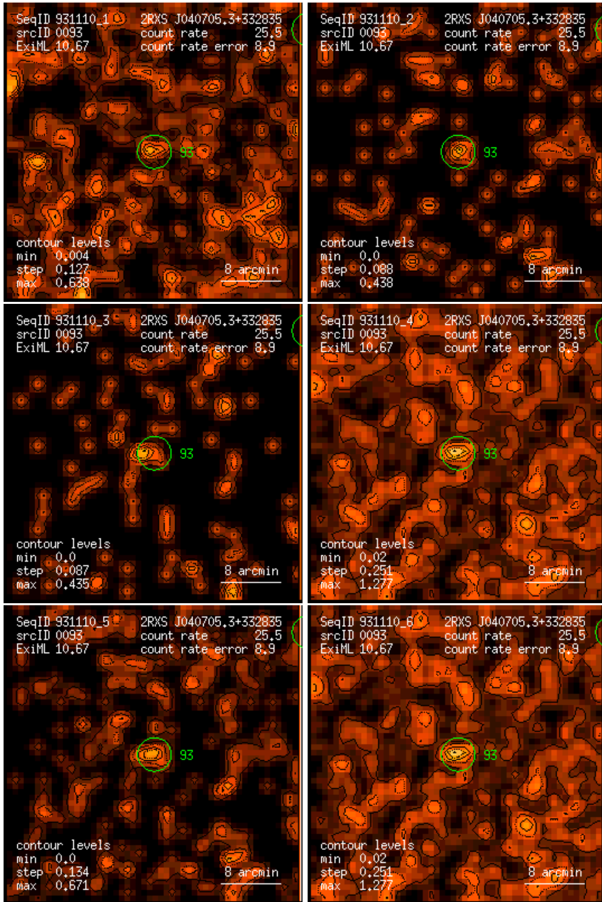
Figure 93: RASS 931110: detection 0093: band rate images, Gaussian filter: (1) PSPC channels 11 – 41, (2) 52 – 90, (3) 91 – 201, (4) 11 – 235, (5) 52 – 201, (6) 11 – 201. Broad band rates in counts/ks. Band rate contour levels in counts/ks/arcmin 2 .
