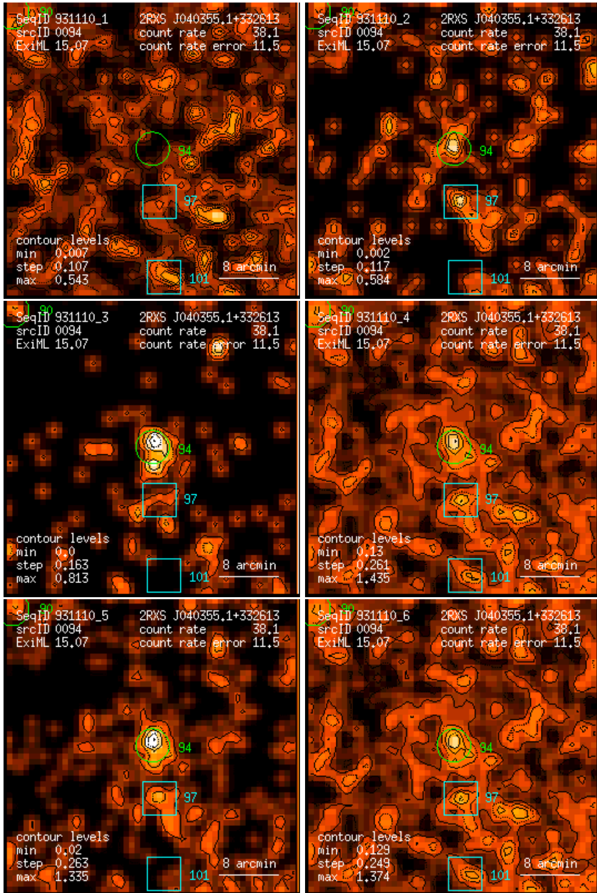
Figure 94: RASS 931110: detection 0094: band rate images, Gaussian filter: (1) PSPC channels 11 – 41, (2) 52 – 90, (3) 91 – 201, (4) 11 – 235, (5) 52 – 201, (6) 11 – 201. Broad band rates in counts/ks. Band rate contour levels in counts/ks/arcmin 2 .
